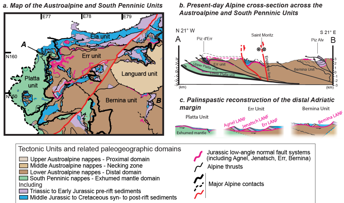
Figure 2: a) Simplified tectonic map along the Central Alps (eastern Switzerland), b) present-day alpine cross-section and c) palinspastic reconstruction of the Adriatic margin, modified from Mohn et al. (2011), Mohn et al. (2012) and McCarthy et al. (2021).
