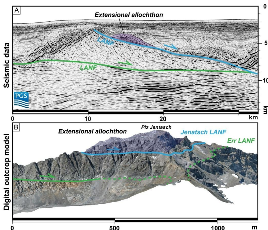
Figure 6: A. Seismic cross-section across a hyper-extended basin in the Southern margin of the South China Sea, modified from Legeay et al., (2024). B. Zoom on the model 11 (Figure 5), where Jurassic rift related extensional structures are observed.
