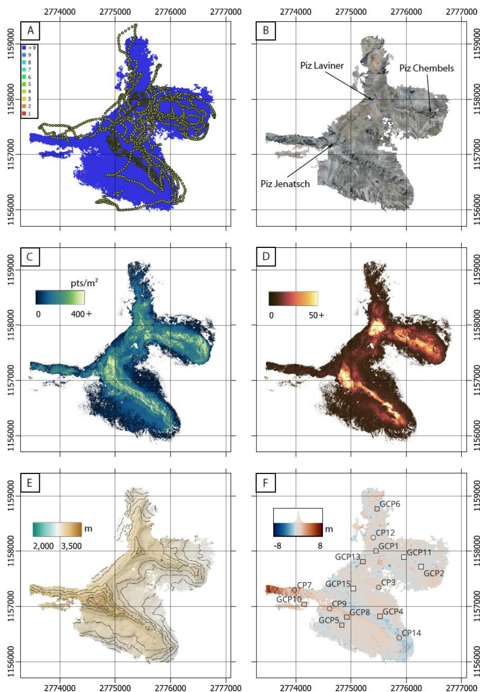
Figure 3: Detailed data overview of Lavinier and Jentasch area DOM (model 11). A. Camera locations (yellow dots) and image overlap indicate good coverage with a majority covered by at least 9 images. B. The Orthomosaic has a spatial resolution of 5 cm/pix. C. The density of the dense cloud ranges from 0 to \geq 400 points/m 2 , lower in the periphery and highest in the center of the model and in steep slopes. D. The confidence, average of all points over a square meter, of the dense cloud ranges from 0 to \geq 50 . E. The Digital Elevation Model (DEM) presents elevation values ranging from 2 680 m to 3 250 m, has a spatial resolution of 10 cm/pixels. F. The DEM comparison map shows the difference between the DEM and regional reference SwissALTI3D DEM.
