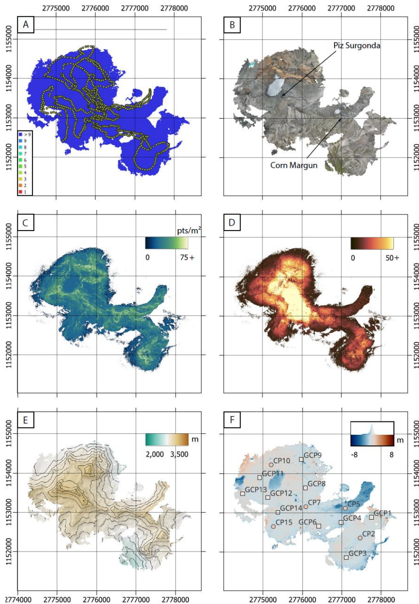
755 Figure A2: Detailed data overview of Piz Surgonda and Corn Margun DOM (model 2). A. Camera locations (yellow dots) and image overlap indicate good coverage with a majority covered by at least 9 images. B. The Orthomosaic has a spatial resolution of 10.9 cm/pix. C. The density of the dense is ranging from 0 to \geq 75 points/m 2 , lower in the periphery and highest in the geological interest outcrops. D. The confidence, average of all points over a square meter, of the dense cloud ranges from 0 to \geq 50 . E. The DEM presents 760 elevation values ranging from 2 050 m to 3 200 m, has a spatial resolution of 21.7 cm/pixels. F. The DEM comparison map based on the reference SwissALTI3D DEM and the histogram of deviation distribution shows that across most of the model, the differences are close to 0, and between -4 and 2 m.
