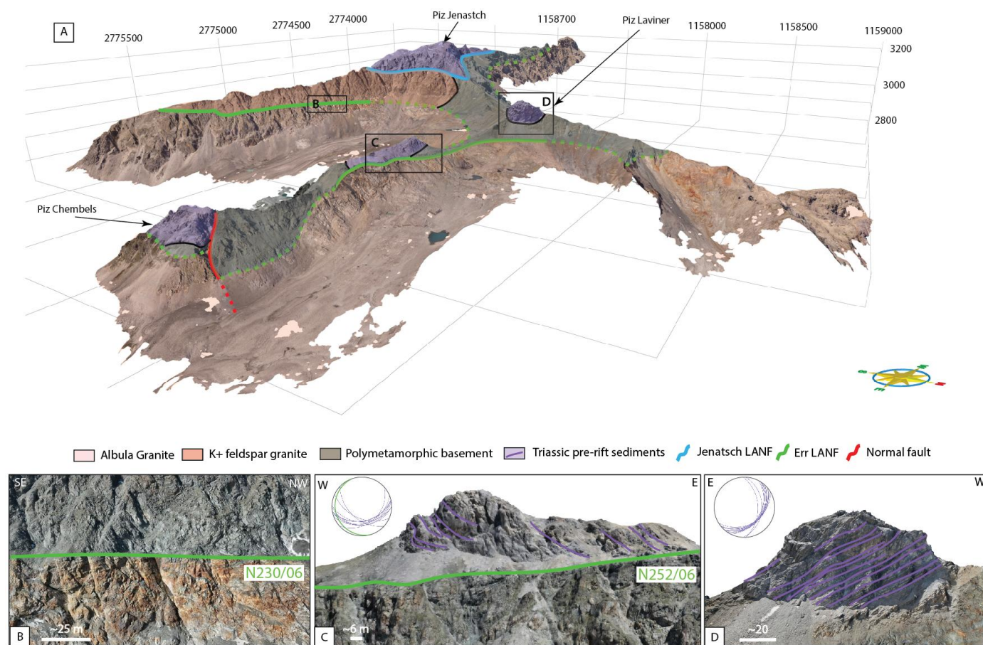
455 Figure 5: The LANFs system in the Laviner and Jenatsch area imaged by the DOM (model 11). A. Large scale interpretation of the model 11 using VRGS. B. Zoom in the Err LANF surface and the damage zone below Piz Jenatsch. C. Extensional allochthonous block on the Err LANF. D. The extensional allochthonous block of Piz Laviner and orientations of structural elements. The stereographic projection in C and D are presented in lower hemisphere Schmidt projection.
