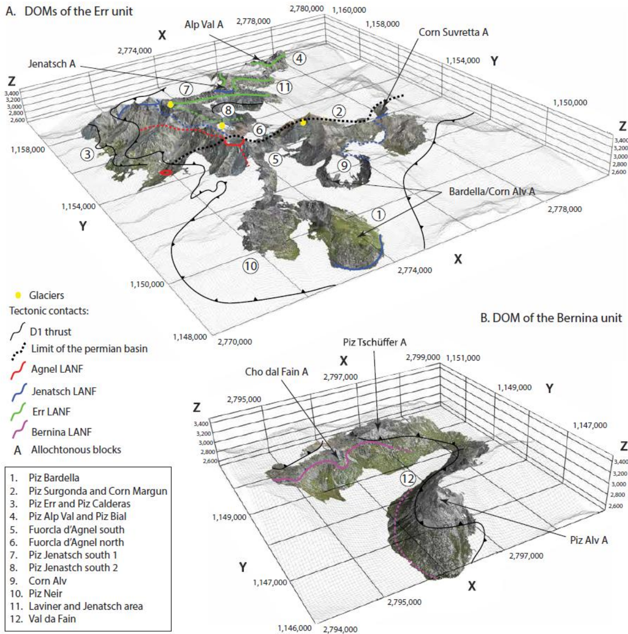
Figure 4: Visualization of the major tectonic contacts in the 12 digital outcrop models of the Err and Bernina units. The tectonic contacts are modified from Epin and Manatschal (2018).
