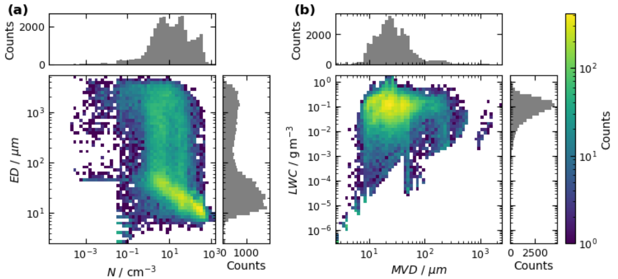
Figure 8. Joint distributions of ED versus N (a) and LWC vs MVD (b) from the cloud encounters during the campaign, color coded by their occurrence.
