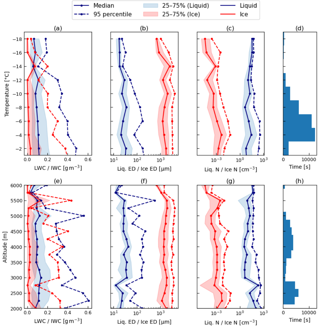
Figure 6. Distribution of (a, e) LWC in blue and IWC in red, (b, f) ED, and (c, g) N observations, sorted into 2°C temperature and 250 m altitude bins. The histogram in (d, h) shows the total frequency of observations per temperature bin for each group. Thicker solid lines represent the median values per temperature bin, while dashed lines indicate the 95th percentile. Shaded areas highlight the interquartile range, covering the 25th and 75th percentiles of the measurements.
