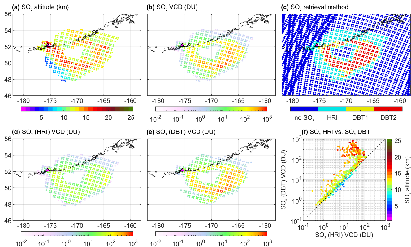
Figure 10. IASI/Metop-A retrievals from 8 August 2008 (morning overpasses) during the Kasatochi eruption. (a) Retrieved \text{SO}_2 altitude. (b) \text{SO}_2 VCDs. (c) Retrieval approach. (d) HRI-based \text{SO}_2 VCDs. (e) DBT-based \text{SO}_2 VCDs. (f) Comparison between HRI-based and DBT-based \text{SO}_2 VCDs, colour-coded by the retrieved \text{SO}_2 altitude. All VCDs and altitudes are in DU and km, respectively.
