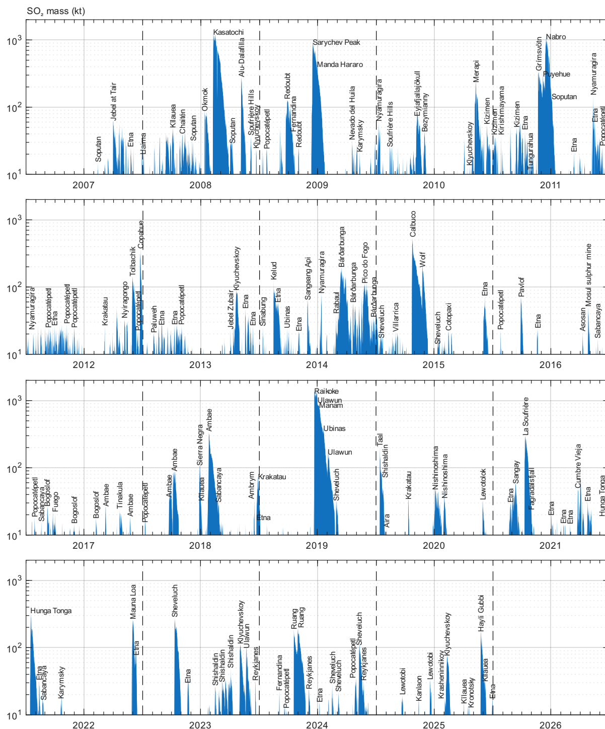
Figure 18. Twice-daily global atmospheric SO 2 masses (in kt) above 5 km altitude derived from IASI observations between July 2007 and December 2025. At each time step, only the maximum SO 2 mass between IASI/Metop-A, -B, and -C (when available) was retained. Major volcanic eruptions detectable with the IASI SO 2 product are indicated (non-exhaustive list).
