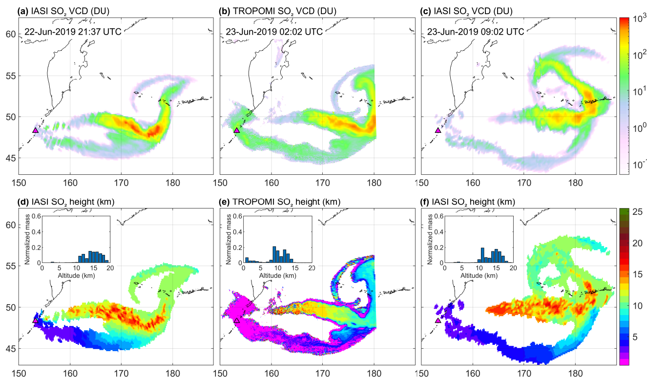
Figure 15. Same as Fig. 13, but during the eruption of Raikoke in June 2019.
