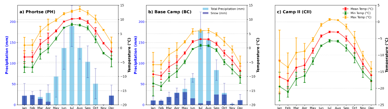
Figure 3. Mean annual cycle of monthly precipitation (snow and total precipitation in mm liquid water equivalent, histograms) and mean monthly mean, minimum and maximum air temperature ( T , lines) during December 2019–November 2022 at PH, BC and CII AWSs. The bar represents the standard deviation for all different variables.
