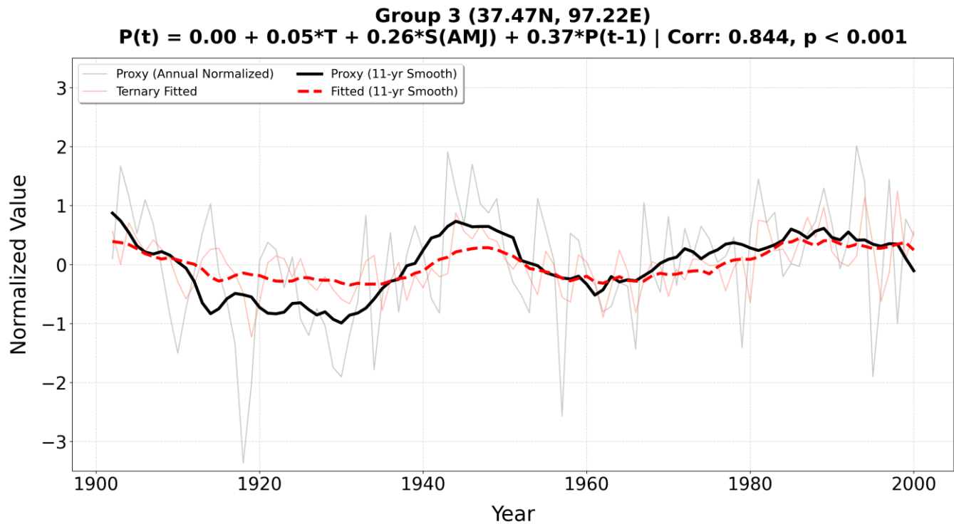
455 Figure 12. Temporal consistency between the actual tree-ring proxy and the TPHH-based ternary fitted series (1901–2000). The fitted series is generated via a standardized ternary regression model integrating TPHH JJA temperature (T), AMJ specific humidity (S), and lag -1 biological memory of the tree-ring proxy (P). Bold lines denote the 11-year moving average, highlighting the low-frequency correlation. See Supplementary Figures S9–S23 for all the validations across 41 proxy groups.
