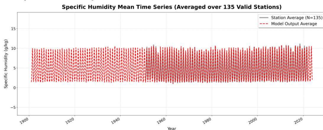
Figure 11. Time series validation with site-observations for temp (a) and shum (b). Shown as the averaged model output (spatial-inferred to sites) joined with the site-observation series.
