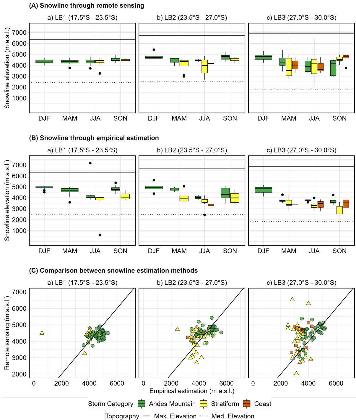
Figure 6. A) Snowline elevation detected through MODIS imagery, and B) estimated empirically in each latitudinal band, and C) estimation scatter plot, categorized by storm during 2000–2019. The Maximum (solid line) and median (dotted line) elevations by band are also included to illustrate the snow-covered area.
