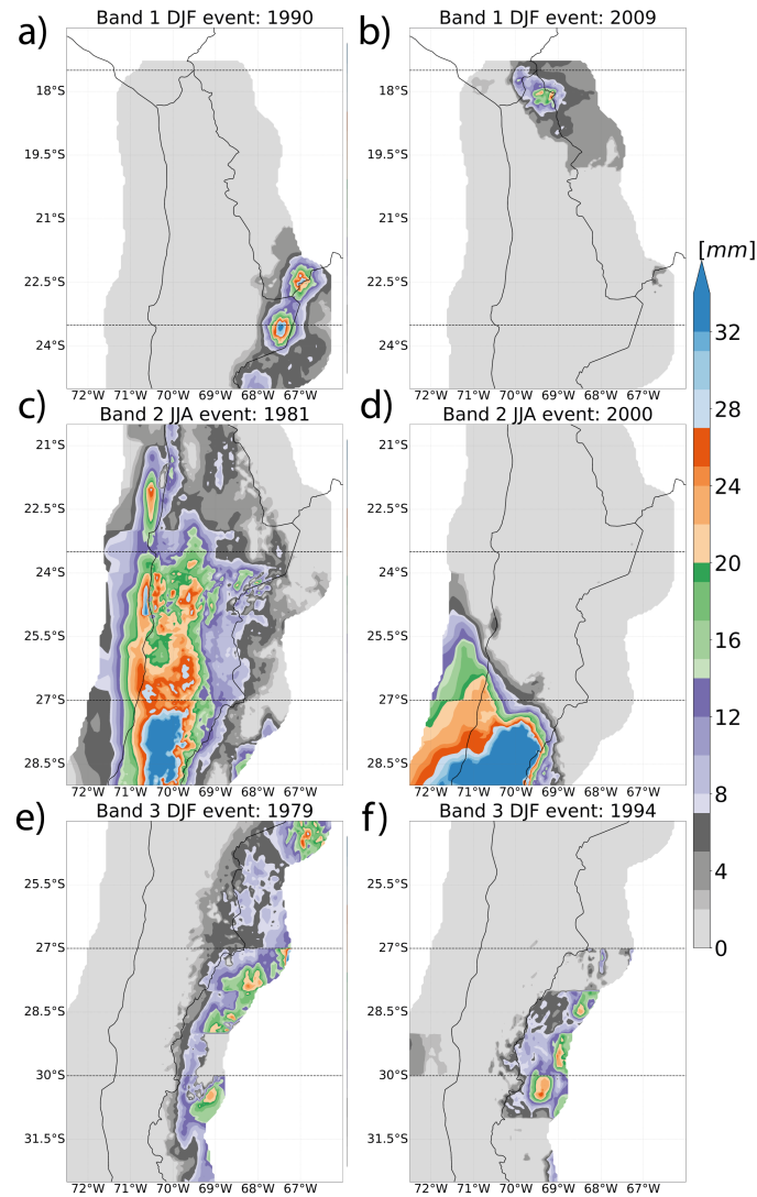
Figure 3. Examples Representative examples of precipitation patterns (mm) for the extreme precipitation events identified in the catalog. selected to display typical patterns for each category . The black rectangle delimits the latitudinal band related to the event. The panels (a) and (b) show the summer events of 1990 and 2009 in LB1, with a Andes Mountain/South Andes and Andes Mountain/North Andes category, respectively; panels (c) and (d) correspond to the winter events of 1981 and 2000 in LB2, with a Stratiform and Coast category, respectively; and the panels (e) and (f) are the summer events of 1979 and 1994 in LB3, with a Andes Mountain/Along Andes category, respectively.
