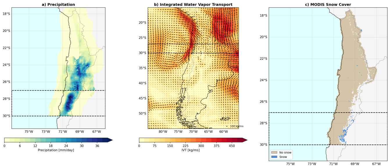
Figure A1. Example reading of the catalog for the LB3 MAM 2015 extreme precipitation event (2015-03-24). (a) Daily precipitation (mm/day) from CR2METv2.5 over the study area (17.25°S–31.5°S, 77°W–66°W). (b) Vertically integrated water vapor transport magnitude (kg/ms; shading) and direction (vectors; reference arrow: 100 kg/ms) derived from ERA5, shown over a broader South American domain (15°S–55°S, 85°W–55°W). (c) MODIS-derived snow cover classification for the event date, distinguishing snow-covered (blue) and snow-free (beige) pixels. Dashed rectangles indicate the LB3 latitudinal band (27°S–30°S).
