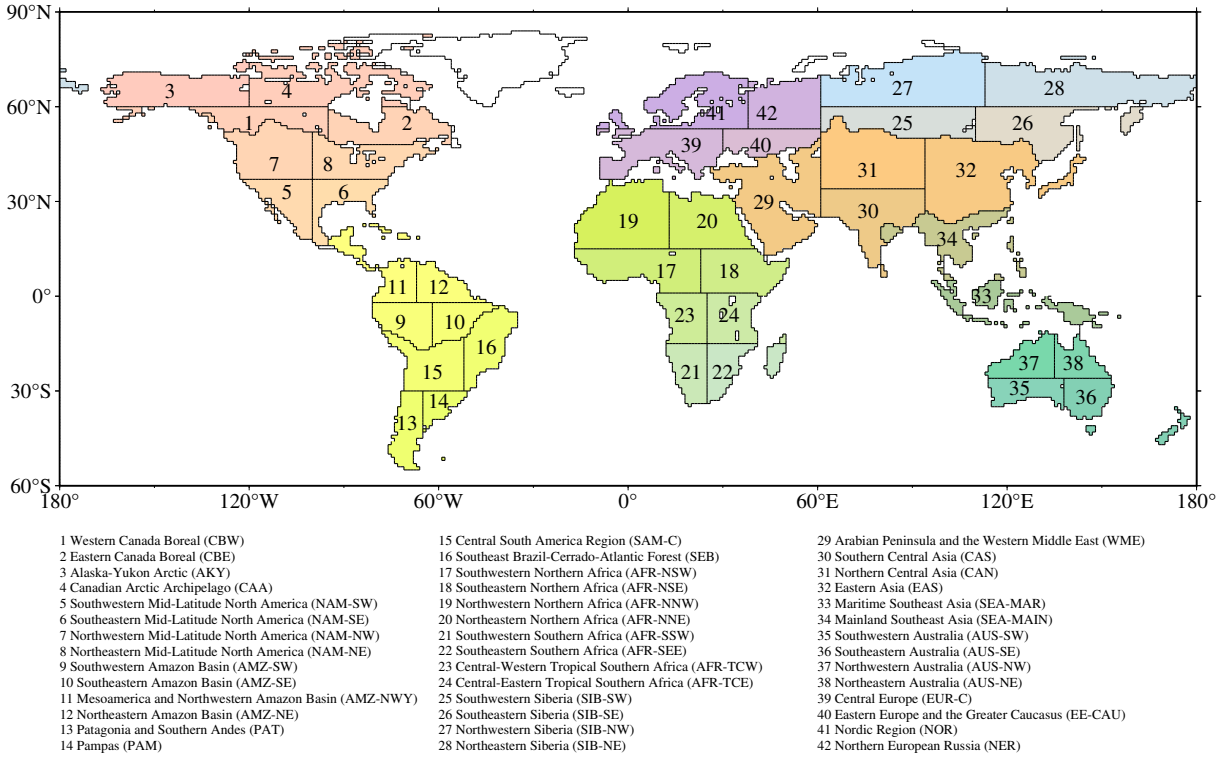
Figure A3. Global land regions used in this study. The land surface is subdivided into 42 spatial units based on geographic location and broad climatic-biogeographic characteristics, following the regional classification adopted in the GOSAT Level 4 product.
