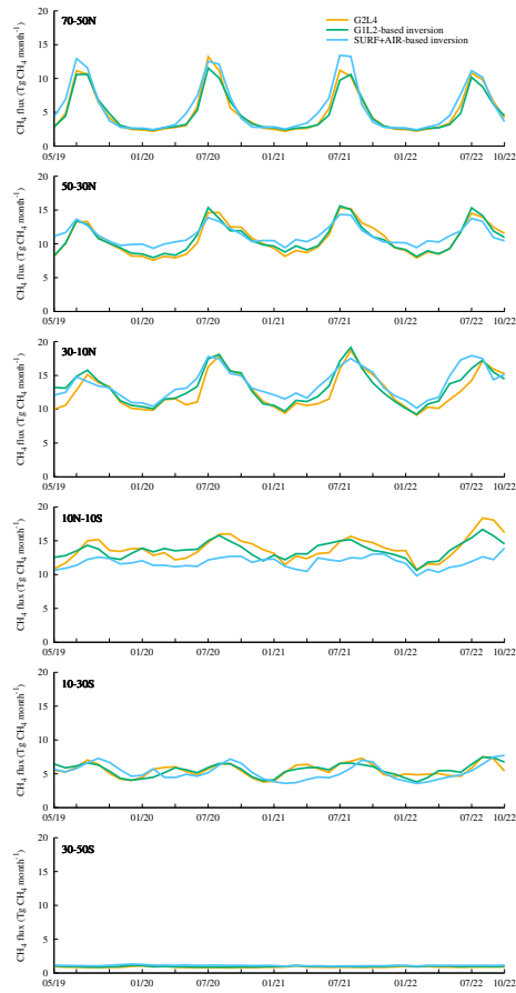
Figure A2. Same as Fig. 6, but showing monthly \text{CH}_4 flux variations ( \text{Tg CH}_4 \text{ month}^{-1} ) estimated from G2L4 (orange), G1L2-based inversions (green), and ground-based inversions (blue).
