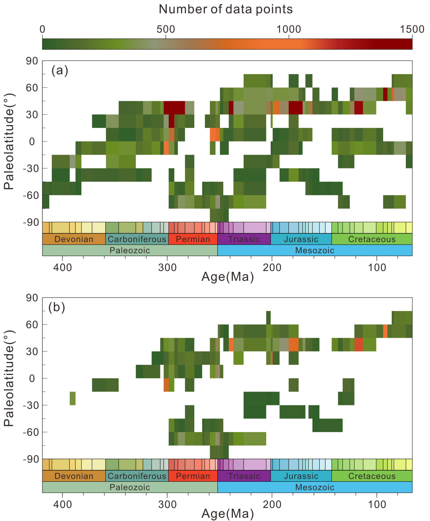
270 Figure 8. Spatiotemporal distribution of the compiled data. (a) Distribution of TOC records over time and across latitudinal bands. (b) Distribution of \delta^{13}\text{C}_{\text{org}} records over time and across latitudinal bands. The colorful boxes on the x-axis represent the stratigraphic framework; see details in the International Chronostratigraphic Chart (v2024-12), ( https://stratigraphy.org/ , last access: 30 December 2025).
