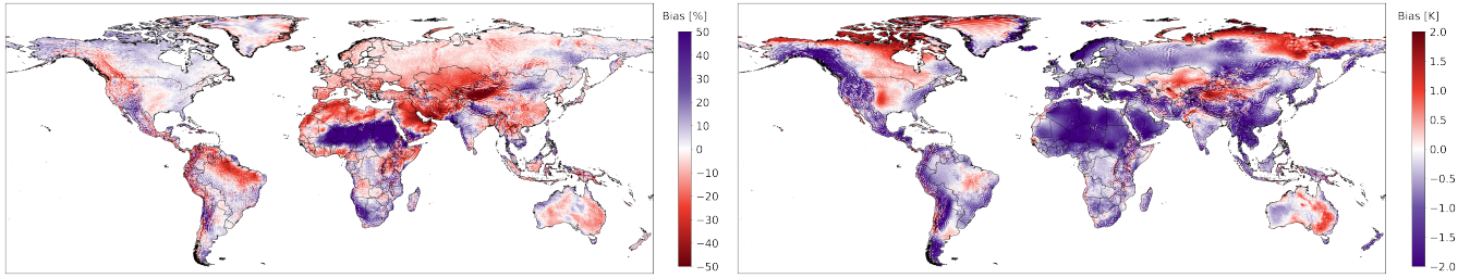
Figure 1. Mean bias of uncorrected SEAS5 (“raw”) forecasts Lead Month 1 relative to ERA5 for precipitation (left) and temperature (right) for the reference period (1981 to 2016). Precipitation bias is shown as relative deviation (%), and temperature bias as absolute deviation (K).
