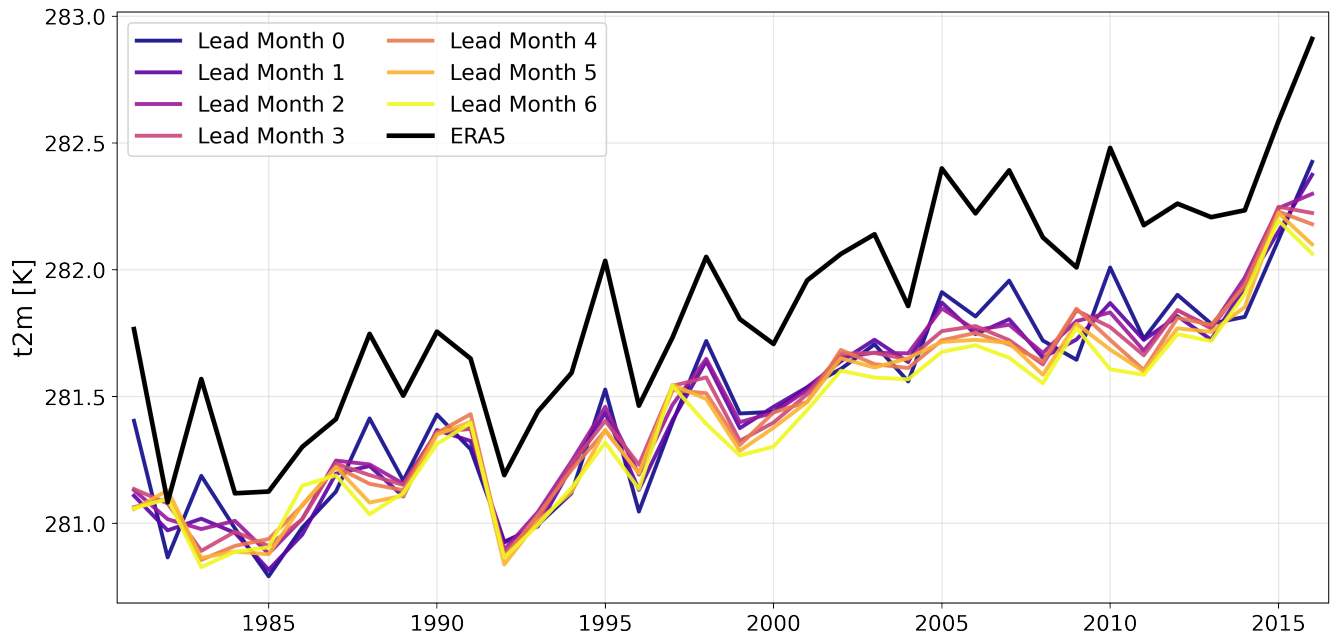
Figure A4. Bias between uncorrected SEAS5 and ERA5 for different lead times. Yearly means across all land masses are shown for the period 1981 to 2016.
