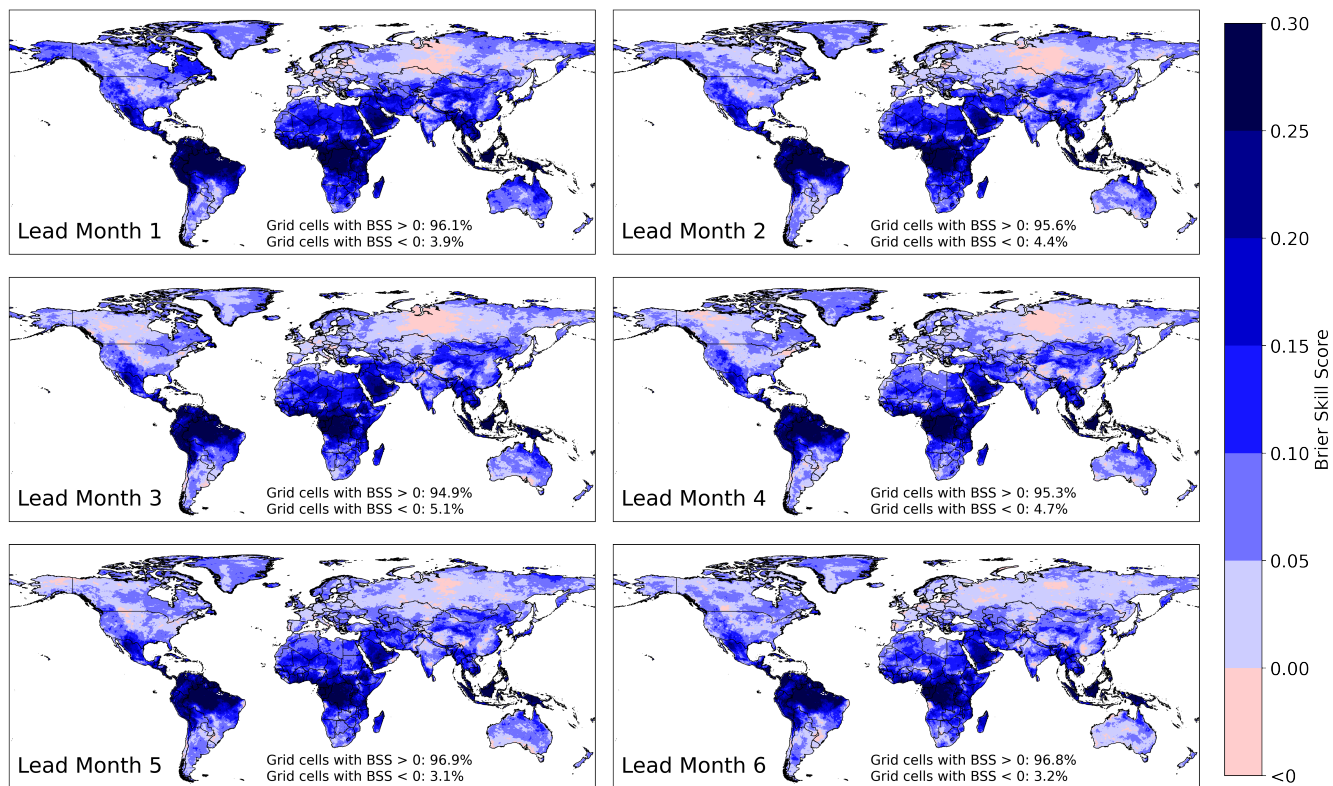
Figure 2. SEAS5-BCSD, Brier Skill Score (BSS) relative to climatology for 2m-temperature, focusing on dry conditions below the 33rd percentile for Lead Months 1–6. Blue colors indicate higher skill than climatology, with darker shades representing better performance.
