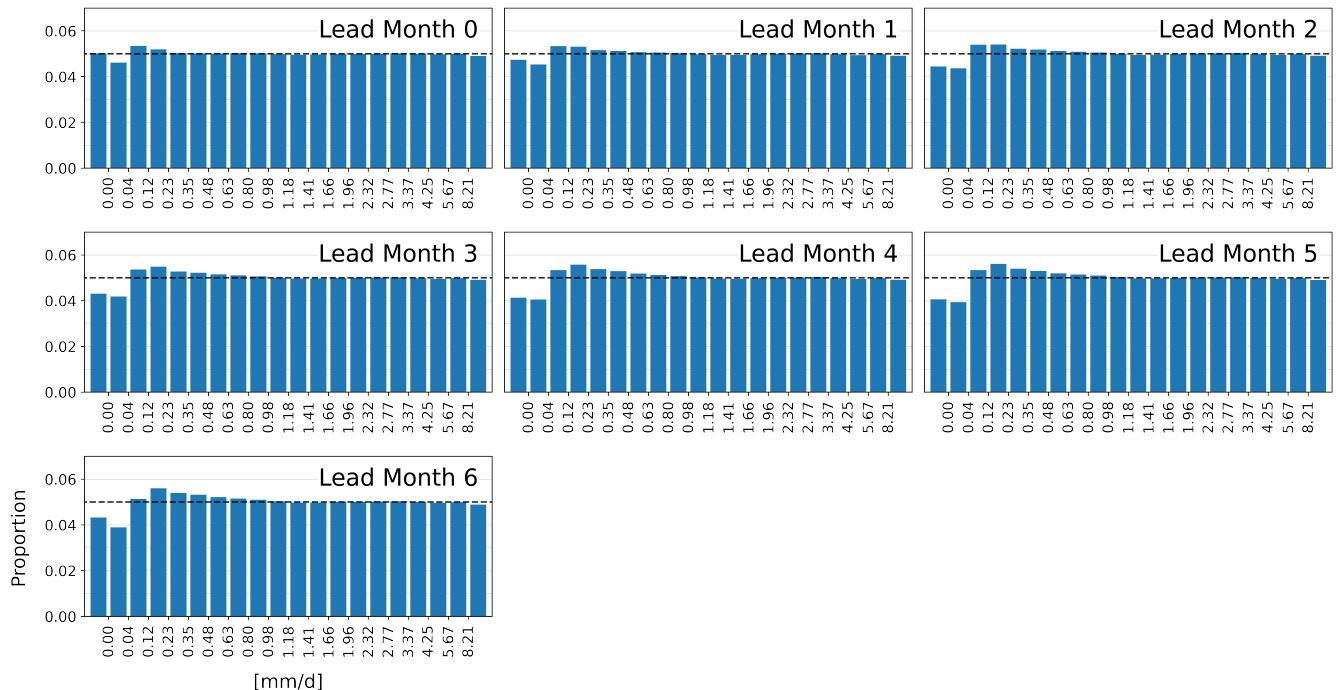
Figure 5. Histogram of BCSO-corrected SEAS5 monthly precipitation values for the period 1981–2016. Bin thresholds are defined by ERA5 percentiles (5th to 95th), such that each bin contains 5 % of the ERA5 data. A uniform distribution of SEAS5 values across bins would indicate perfect agreement with the ERA5 reference distribution.
