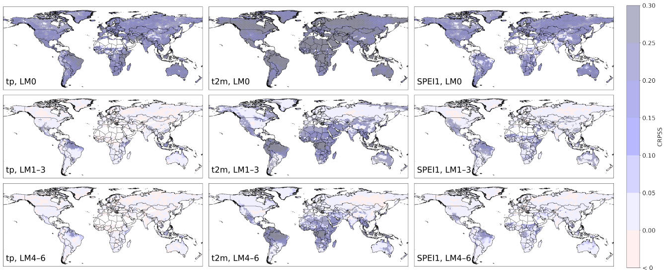
Figure 5. SEAS5-BCSD, Continuous Ranked Probability Skill Score relative to climatology for different lead months (LMs), shown for precipitation (left) and temperature (middle) and SPEI-1 (right). Lead Month 0 (top), Lead Months 1–3 (middle), and Lead Months 4–6 (bottom) are displayed. Dry grid cells are excluded. Hatching indicates grid cells where the lower bootstrap bound exceeds zero ( p > 0.95 ).
