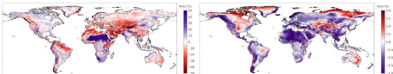
Figure 1. Bias-Mean bias of uncorrected SEAS5 (“raw”) forecasts Lead Month 1 relative to ERA5 for precipitation (left) and temperature (right) for the reference period (1981 to 2016) . Precipitation bias is shown as relative deviation (%), and temperature bias as absolute deviation (K).
