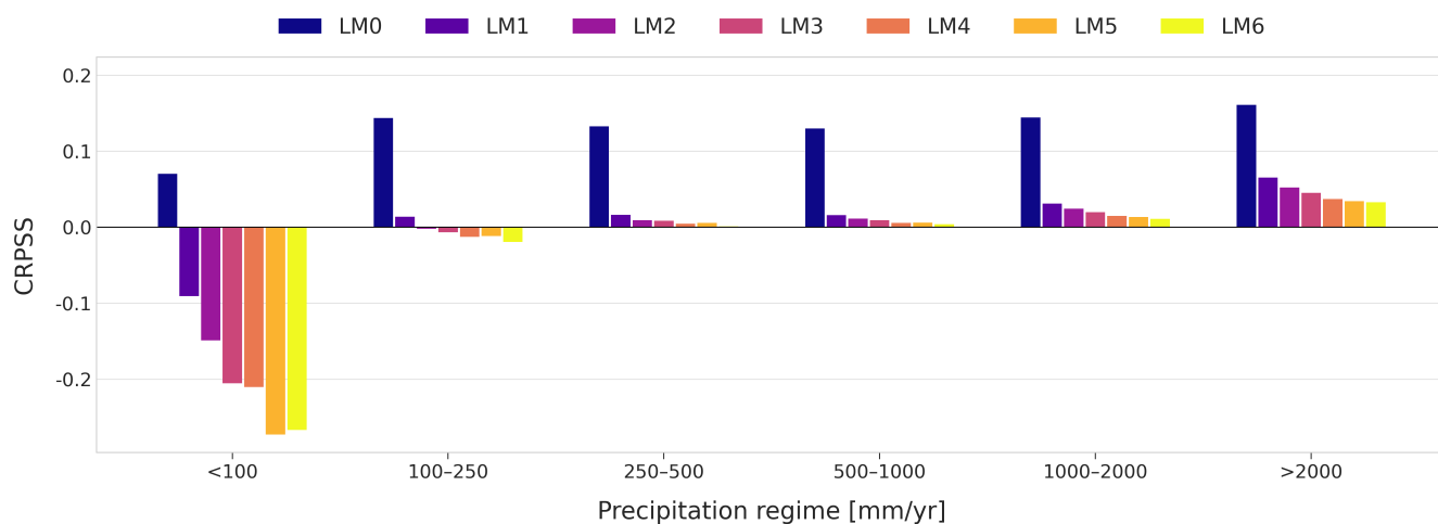
Figure 3. SEAS5-BCSD, yearly mean precipitation sum compared to the Continuous Ranked Probability Skill Score (CRPSS) relative to climatology. The area is grouped by precipitation thresholds into 6 bins, each showing seven lead months.
