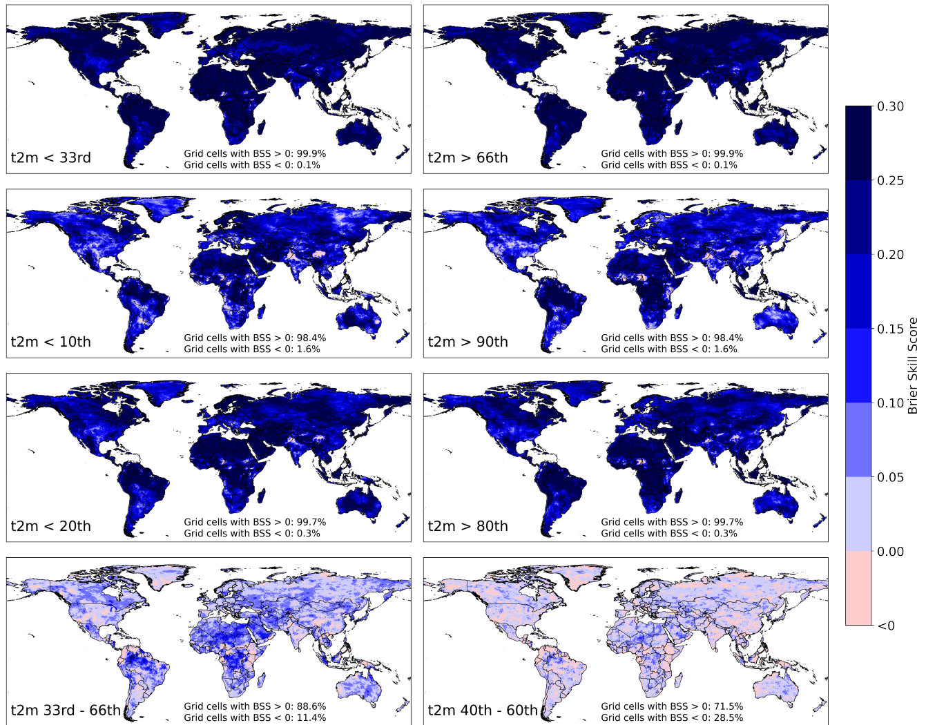
Figure 1. SEAS5-BCSD, Brier Skill Score (BSS) relative to climatology for 2m-temperature at Lead Month 0. Different percentile thresholds are shown, indicated in the lower-left corner of each panel. Blue colors indicate higher skill than climatology, with darker shades representing better performance.
