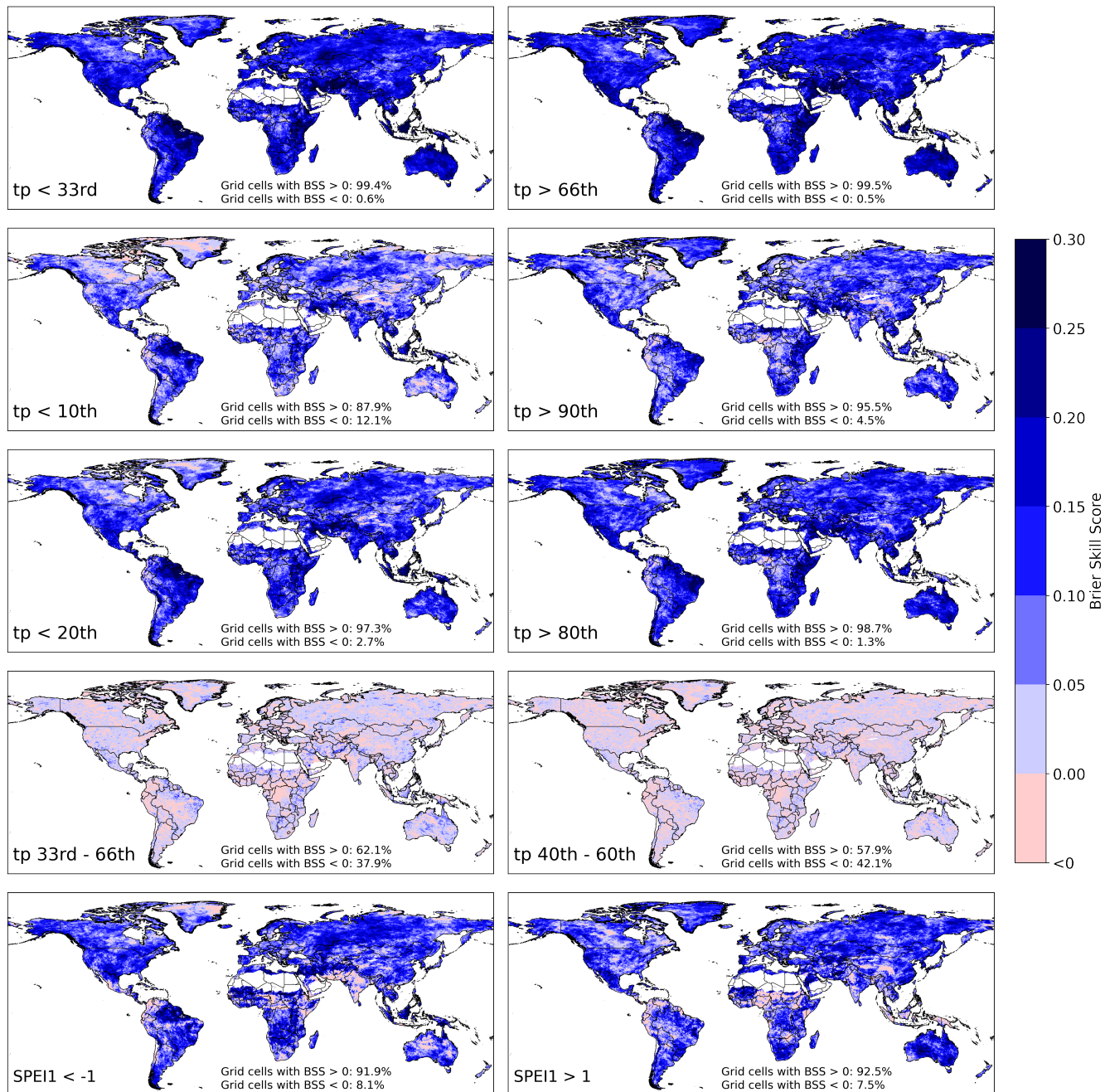
Figure 3. SEAS5-BCSD, Brier Skill Score (BSS) relative to climatology for precipitation, as well as SPEI-1 , at Lead Month 0. Different percentile thresholds are shown, indicated in the lower-left corner of each panel. Blue colors indicate higher skill than climatology, with darker shades representing better performance. Dry grid cells are excluded.
