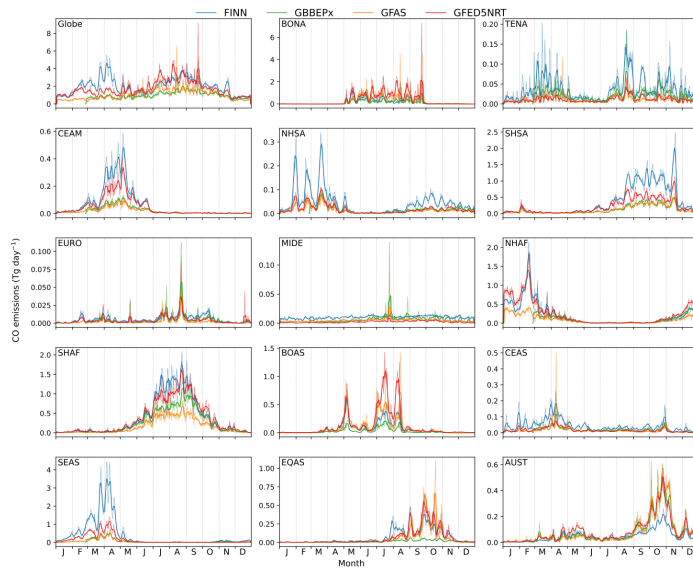
422 423 Figure 7. Comparison of daily global and regional CO emission totals in 2023 from GFED5NRT with three existing 424 daily fire emissions datasets: the Fire Inventory from NCAR (FINN, v2.5), the Blended Global Biomass Burning 425 Emissions Product (GBBEPx, v3), and the CAMS Global Fire Assimilation System (GFAS, v1.2). Light-colored lines 426 show the original daily time series, and the dark-colored lines show the 5-day smoothed time series.
