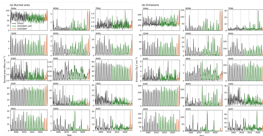
Figure 4. Monthly time series of regionally summed (a) burned area ( \text{Mha mo}^{-1} ) and (b) fire emissions ( \text{Tg C mo}^{-1} ) from GFED5 (2002-2022; black lines) and GFED5NRT (derived from SNPP and NOAA-20 combined, 2023-2024; orange lines). For comparison, the time series of GFED5NRT derived using SNPP only (GFED5NRT_VNP, 2012-2024; green lines) is also shown.
