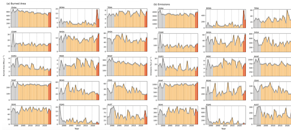
443 444 Figure 8. Annual time series of regionally summed (a) burned area (Mha yr -1 ) and (b) fire emissions (Tg C yr -1 ), 445 merging three GFED5 products: the core period (2002-2022, orange), the pre-MODIS period (1997-2001, gray), and 446 the GFED5NRT product (2023-2024, red).
