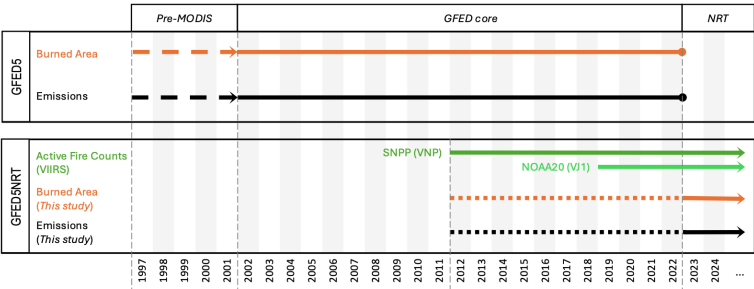
Figure 1. Timelines of GFED5NRT products and primary input datasets. Layers shown include VIIRS active fire counts, burned area, and fire emissions. The dashed lines for GFED5 denotes the pre-MODIS period, when data were reported at coarser spatial resolution. Dotted lines for GFED5NRT denote the periods used for data calibration and for deriving scaling coefficients.
