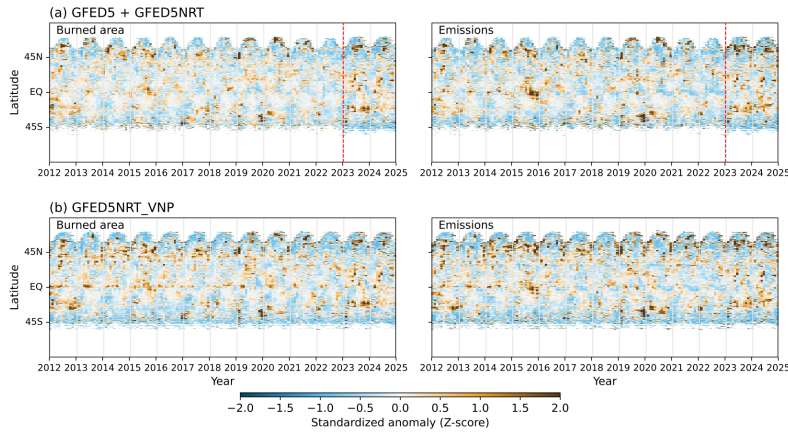
Figure 6. Monthly Z-score of burned area (BA) and fire emissions (EM) in each 0.25° latitudinal band. (a) GFED5 (2012-2022) and GFED5NRT (SNPP and NOAA-20 combined version; 2023-2024). Red dashed vertical lines denote the start of the GFED5NRT record in 2023. (b) GFED5NRT derived using SNPP only (GFED5NRT_VNP) for 2012-2024. The unitless Z-score, or the normalized anomaly, is defined as Z = (v-m)/std , where v is the monthly burned area, m is the climatological monthly mean, and std is the standard deviation of interannual variability. The same climatological means and standard deviations from GFED5 (2012-2022) were used for the calculations of Z-scores in all three datasets.
