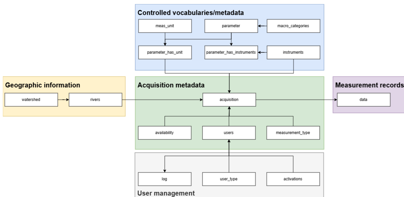
Figure 1 Relational schema of the database PostgreSQL
