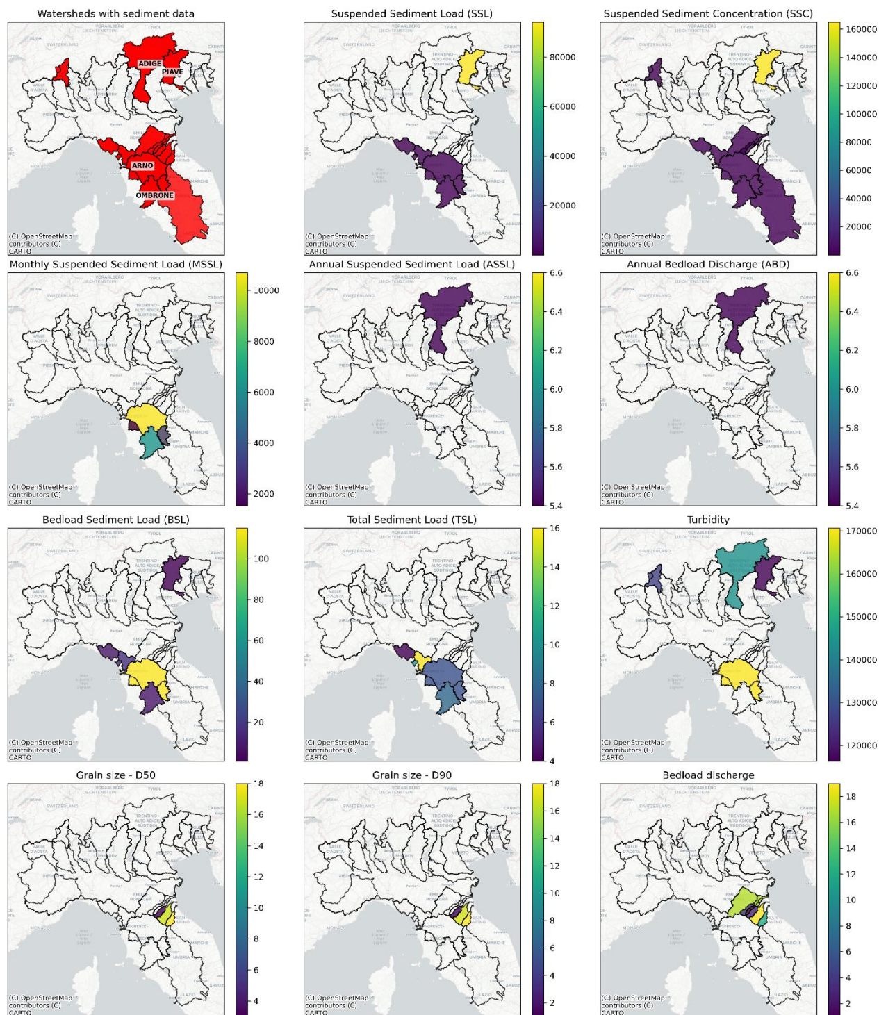
Figure 10 Spatial distribution of sediment transport data for each parameter considered. In the top-left panel, red basins indicate watersheds containing at least one sediment transport parameter, while the remaining basins, outlined in black, are included in the database but associated only with other types of parameters. The other panels show, for each sediment-related parameter, the number of available records within each basin. Colour scales are panel-specific and should not be directly compared across parameters; in each panel, colours represent the number of available records for the corresponding parameter.
