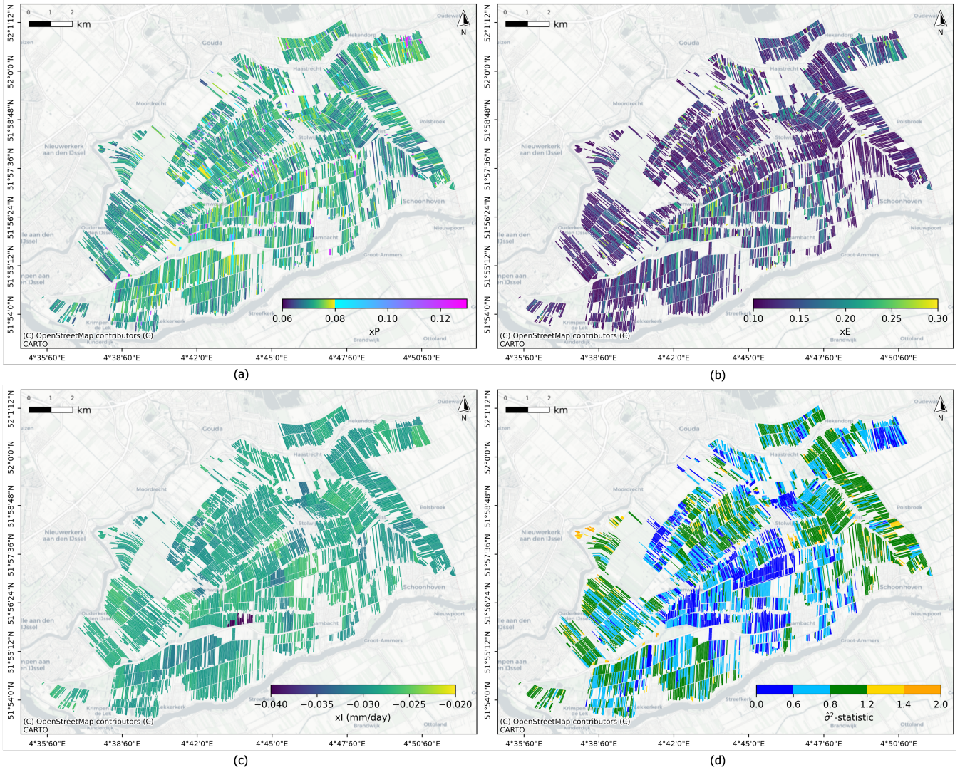
Figure 3. Spatial distributions of the SPAMS parameters for each parcel: (a) scaling factor of precipitation \hat{x}_P , (b) the scaling factor of evapotranspiration \hat{x}_E , and (c) the irreversible scaling factor \hat{x}_I in mm/day. Panel (d) shows the \hat{\sigma}^2 test statistic values of each parcel. The parameters are estimated from InSAR observations from 2015 to 2025, using precipitation and evapotranspiration data from the closest meteorological station for each parcel centroid. Note that (c) alone should not be used directly to estimate the annual subsidence rates
