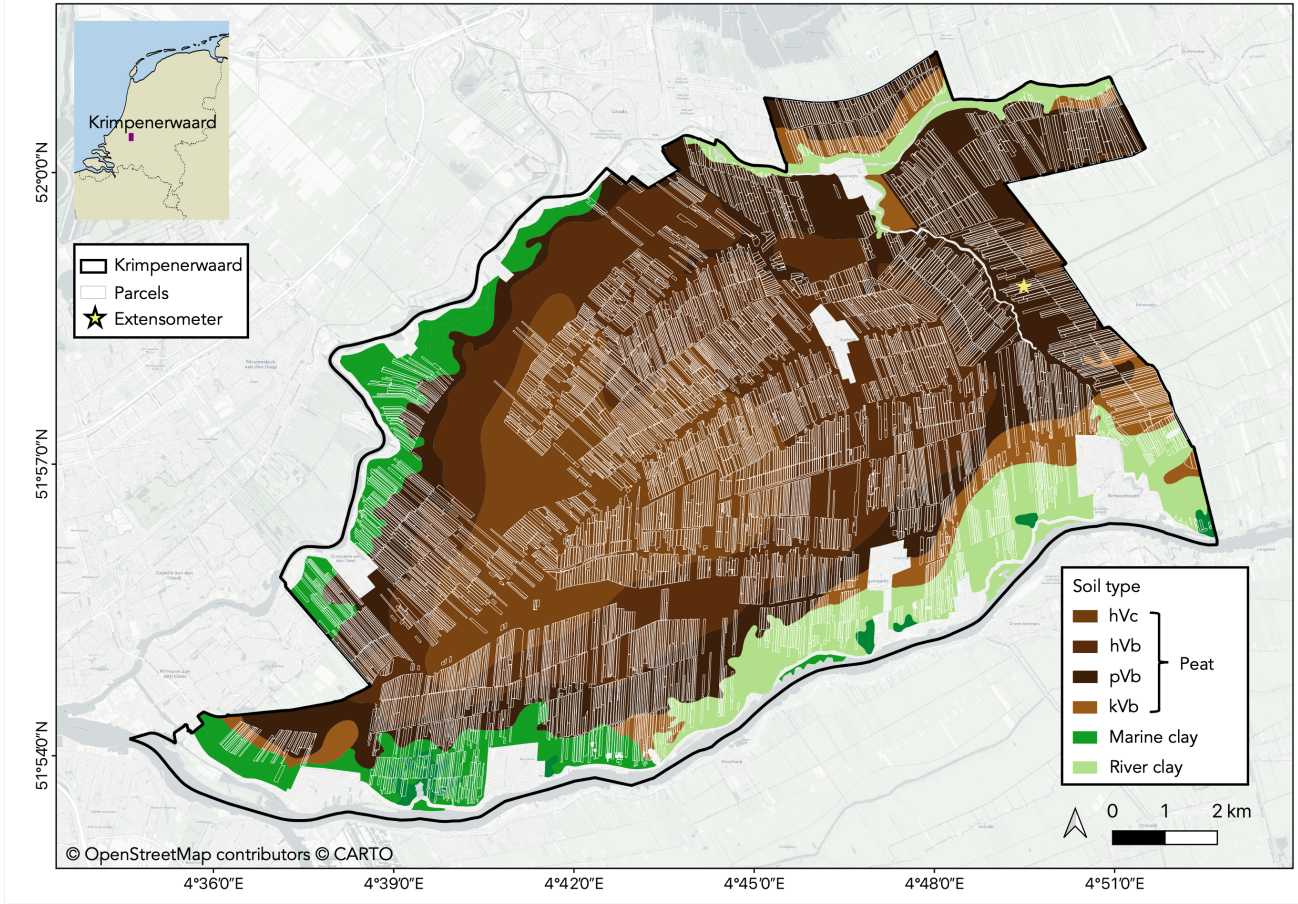
Figure 2. Spatial distributions of Krimpenerwaard study area overlaid with the sealing factor of precipitation \hat{x}_P (a), the sealing factor of evapotranspiration \hat{x}_E (b), the subsidence rate \hat{x}_I in mm/day (c), soil map and \hat{\sigma}^2 test statistic (d) parcel polygons having the estimated SPAMS10 parameters. The extensometer site is used for validation purpose.
