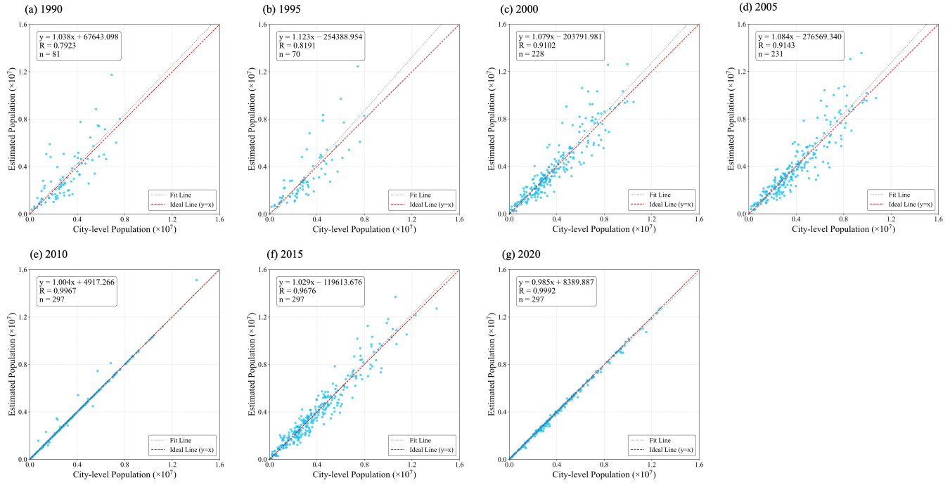
Fig. 6 Multi-temporal evaluation of AGPC gridded population estimates against city-level population statistics
