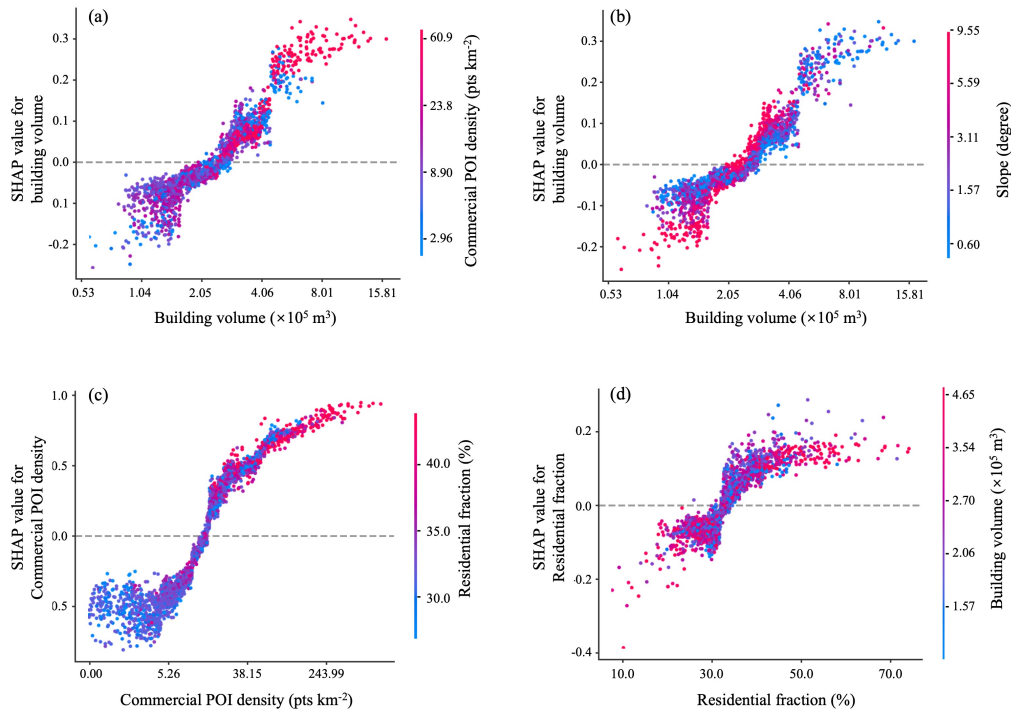
Fig. 11 Dependence plots of covariates identified by the SHAP summary analysis for 2010
