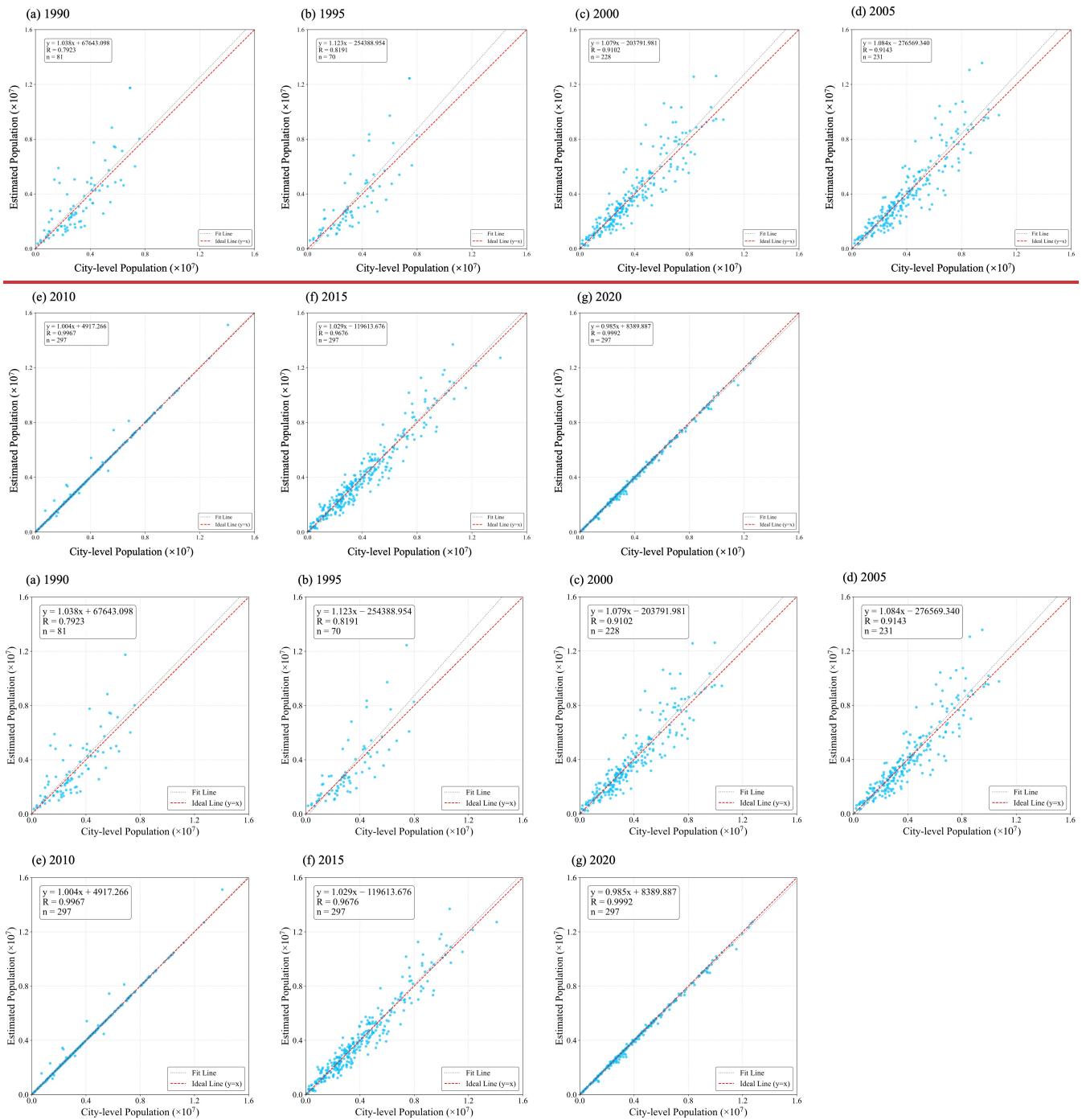
Fig. 6 Multi-temporal evaluations of AGPC gridded population estimates at against city-level population statistics
