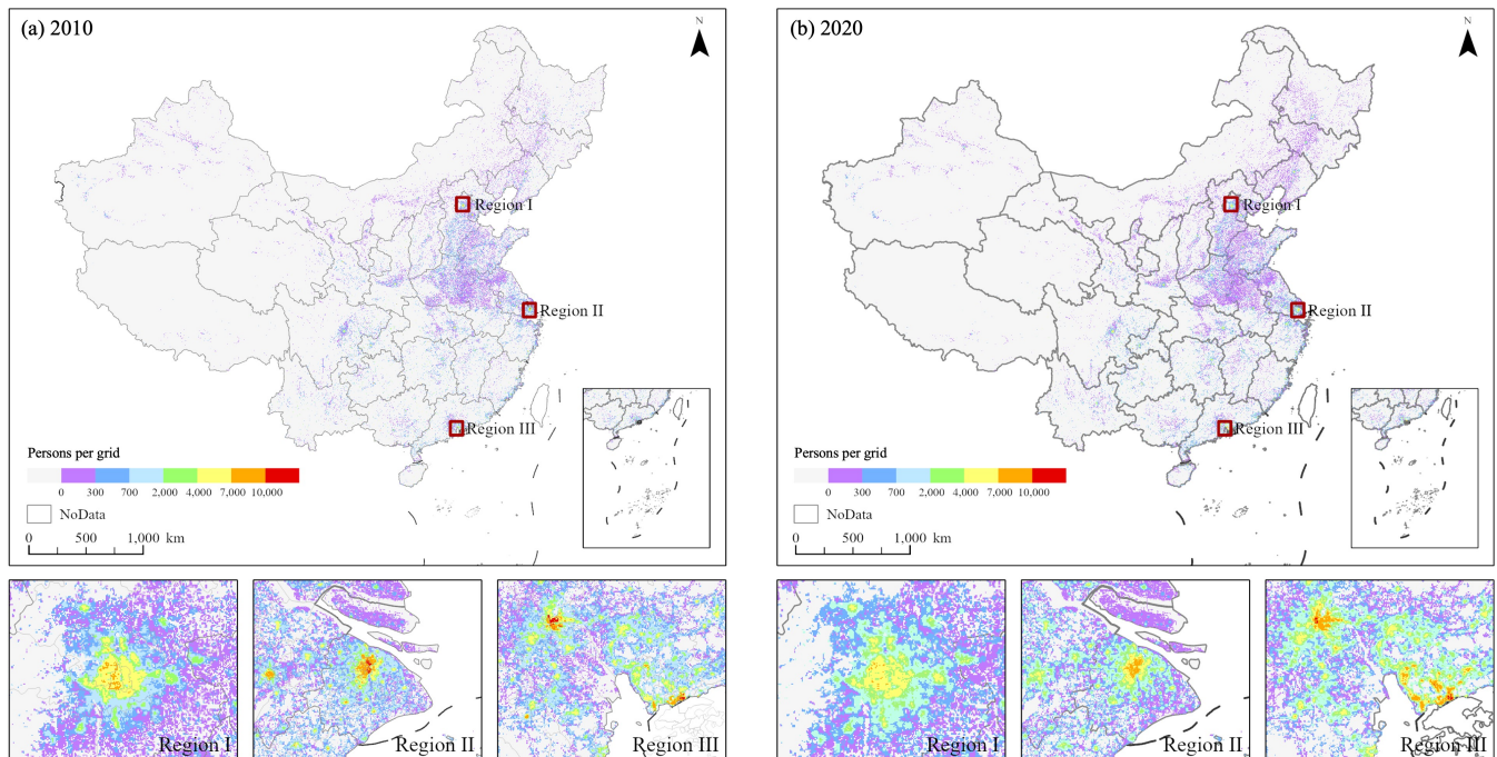
Fig. 8 Spatial distribution of AGPC The 500-m-gridded gridded population estimates at 500 m for China in for 2010 (a) and 2020 (b) in AGPC dataset
