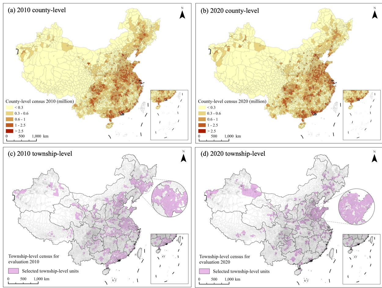
205 Fig. 1 Population census data from Sixth and s Seventh National Population Census of China, including county-level population data for in 2010 (a) and 2020 (b), and the spatial distribution of selected town ship -level census units for population in 2010 (c) and 2020 (d)
