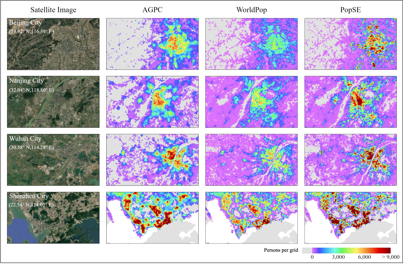
Fig. 13 Comparison of gridded population distributions in 2020 among AGPC, WorldPop, and PopSE in selected areas
