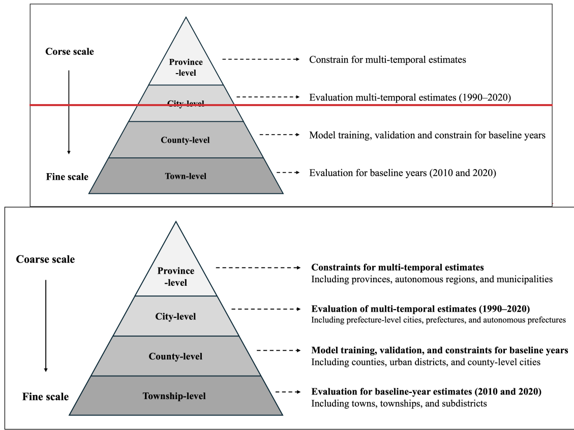
Fig. 2 Hierarchy of population census data and their respective roles in this study roles in model development, population constraints, and evaluation
