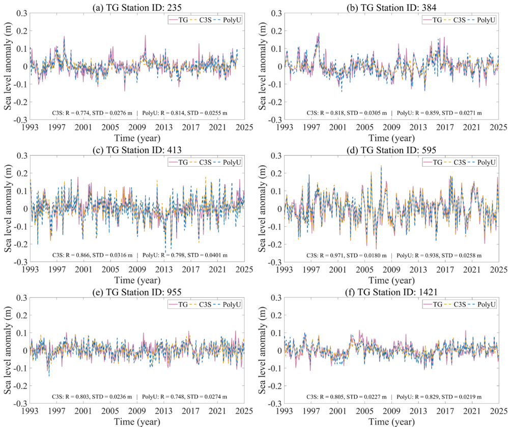
560 Figure 10. Detrended and deseasoned SLA time series from TG, PolyU, and C3S gridded SLA products at selected stations identified in Fig. 9, illustrating cases with different levels of variance differences. The reported correlation coefficients (R) and standard deviations (STD) are computed from these processed time series.
