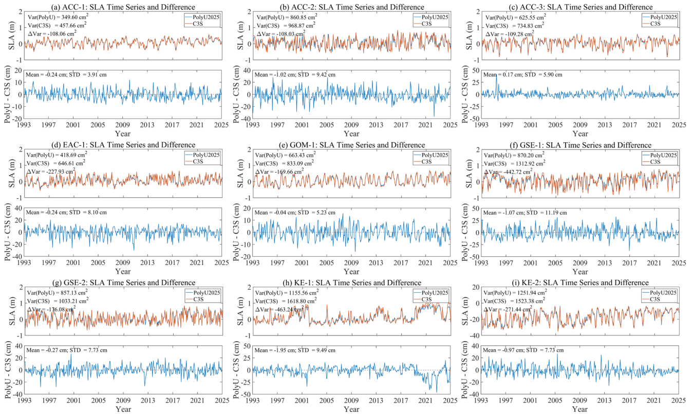
495 Figure 8. SLA time series and their differences between the PolyU and C3S gridded SLA products at nine selected points (locations shown in Fig. 5).
