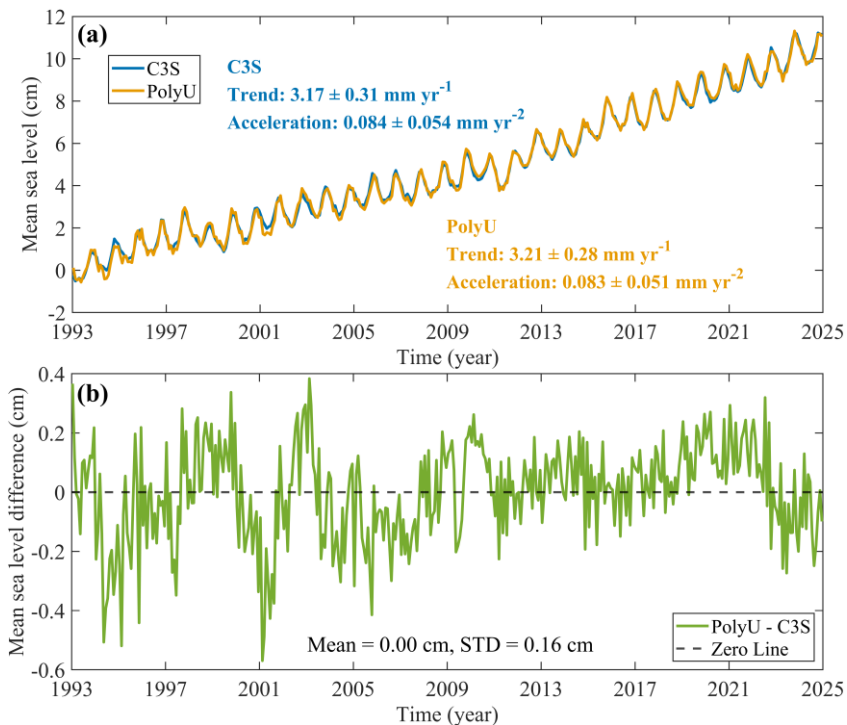
435 Figure 6. Temporal evolution of the global mean sea-level (GMSL) trend estimated from the PolyU (orange line) and C3S (blue line) gridded SLA products over the period from January 1993 to December 2024. The trend was computed with no GIA correction applied. (a) GMSL time series. (b) GMSL difference (PolyU – C3S).
