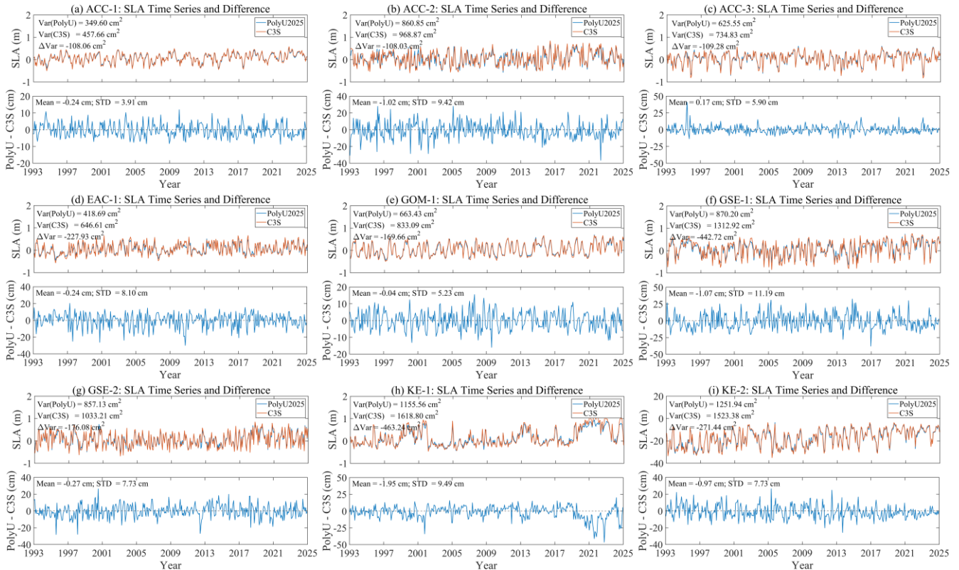
505 Figure 8. SLA time series and their differences between the PolyU and C3S gridded SLA products at nine selected points (locations shown in Fig. 5).
