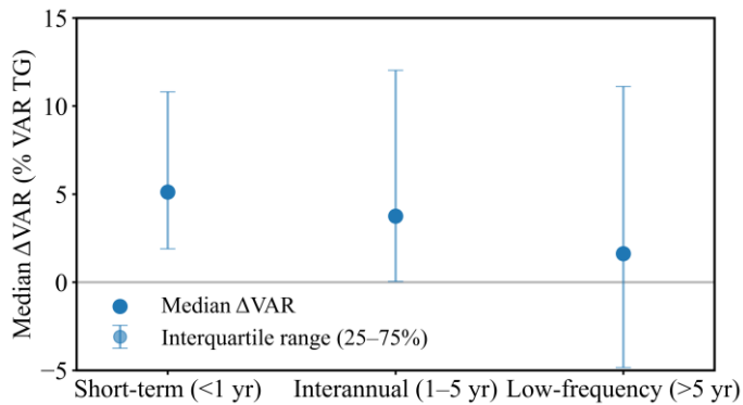
585 Figure 11. Scale dependence of SLA–TG residual variance differences between PolyU and C3S gridded SLA products. The relative variance difference ( \Delta VAR) is defined as the difference in variance between PolyU–TG and C3S–TG residuals, normalized by the variance of the TG observations, and expressed as a percentage. Results are presented for three temporal scales: short-term (<1 year), interannual (1–5 years), and low-frequency (>5 years). Dots represent the median \Delta VAR across stations, and error bars indicate the interquartile range (25th–75th percentiles).
