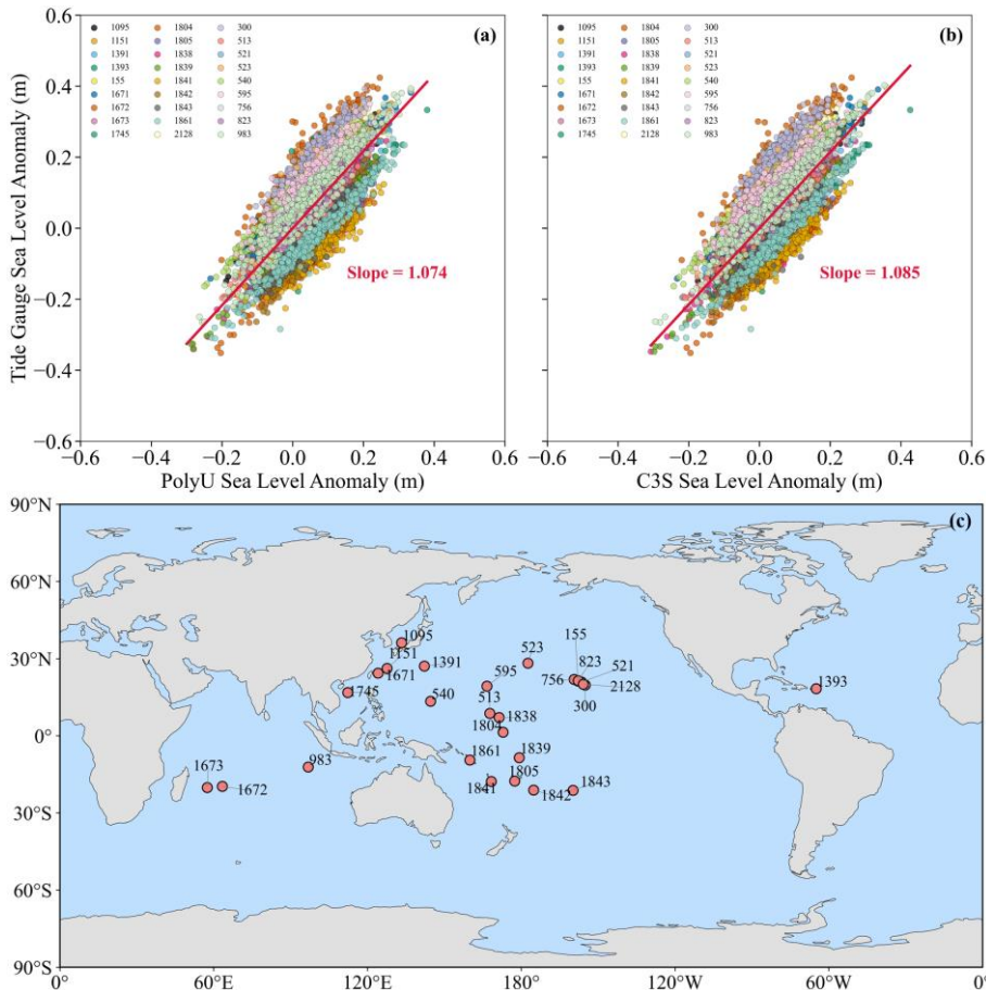
665 Figure 13. Comparison of SLA from the PolyU and C3S gridded SLA products with TG observations at 27 open-ocean TG stations. (a) Scatter plot of SLA from the PolyU gridded SLA product versus TG observations. (b) Scatter plot of SLA from the C3S gridded SLA product versus TG observations. (c) Geographical distribution of the 27 selected TG stations, with station identifiers from the PSMSL database.
