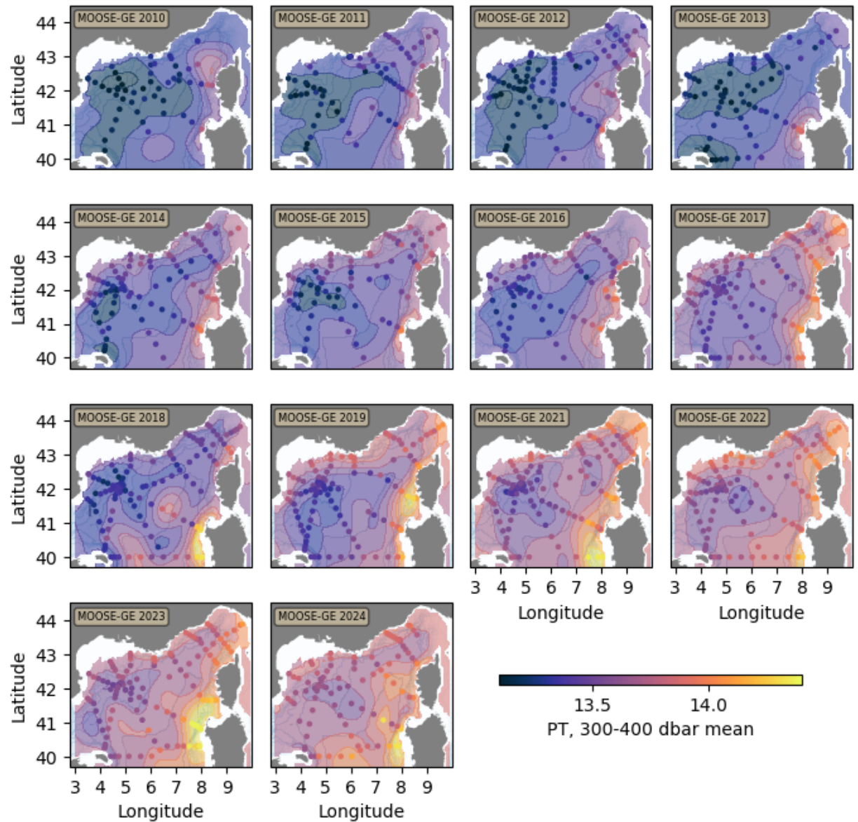
Figure 3: Maps of the spatial distribution of potential temperature in the 300–400 dbar layer, representative of the Levantine Intermediate Water (LIW), in the northwestern Mediterranean Sea basin for each MOOSE-GE cruise from 2010 to 2024. The background field corresponds to an optimal interpolation (correlation length scale of 100km) of the station observations, which are shown as colored dots.
