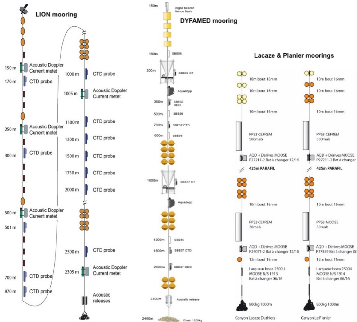
846 Figure 2: Moorings design of LION, DYFAMED, Lacaze and Planier deployed in the northwestern 847 Mediterranean Sea region
