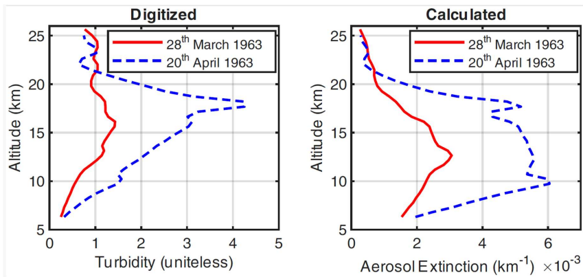
Figure 2: Plots of the digitized ATP (left panel) and the calculated AEP (right panel) for March 28 and April 20, 1963.
