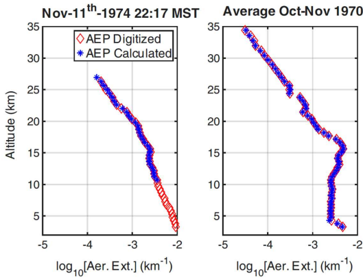
240 Figure 1: Plot of the digitized and calculated AEP from the November 11th 1974 at 22:17 MST and October 2 November 1970 average profiles, reported in plots in Elterman (1975) and Elterman et al. (1973) respectively. Both pairs of digitized AEPd and AEPc show good agreements.
