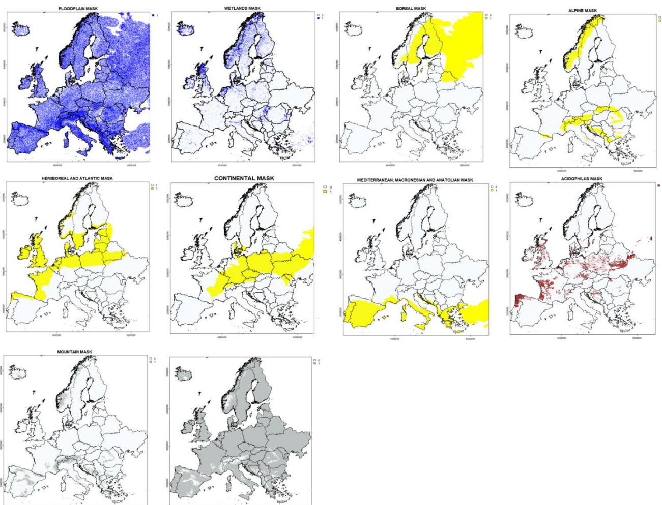
300 Figure 2. Environmental “Breaking point” forest masks for EFTs classification.
