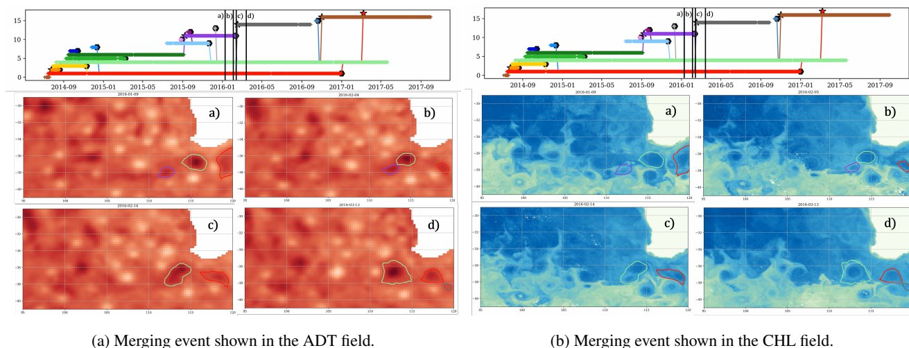
Figure 18. Merging event observed in both ADT and CHL fields (between purple and light green eddies).
