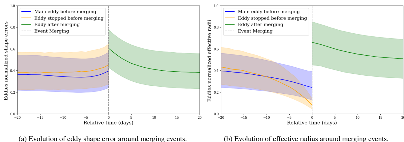
Figure 13. Median and interquartile range of eddy normalized shape error and effective radius around merging events.
