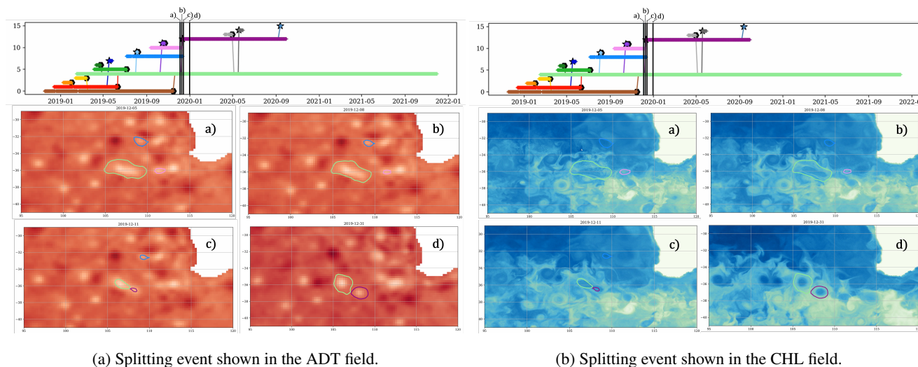
Figure 19. Splitting event observed in both ADT and CHL fields (purple and light green eddies).
