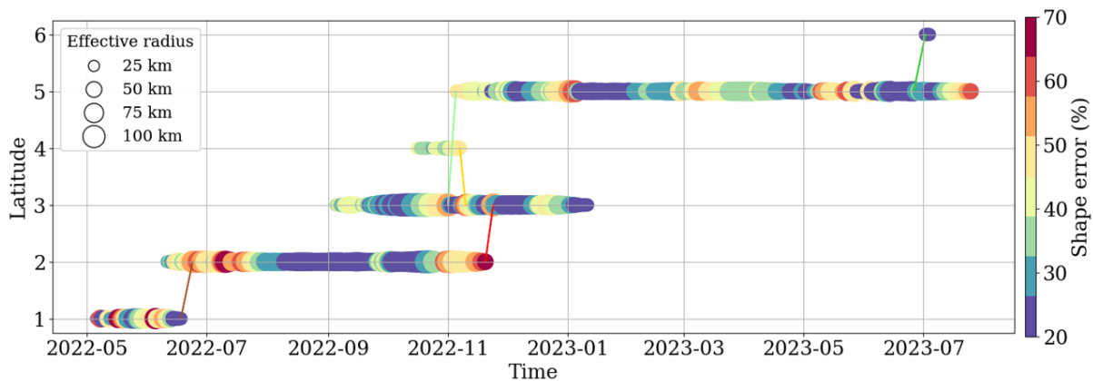
Figure 4. Timeline of eddy trajectories. Marker color indicates shape error, while marker size is proportional to eddy radius.
