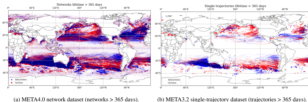
Figure 10. Comparison of eddy trajectories persisting longer than 365 days in META3.2 and META4.0. META4.0 exhibits more long-lived trajectories than the single-trajectory dataset, particularly in regions of strong eddy activity.
