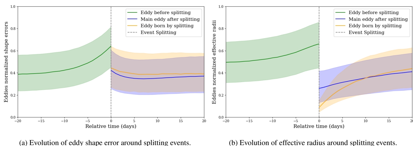
Figure 14. Median and interquartile range of eddy normalized shape error and effective radius around splitting events.
