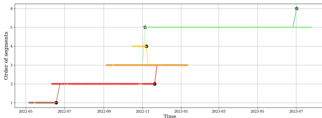
(a) Demo network timeline function of the segments' orders.
