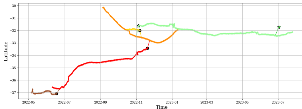
(b) Demo network timeline function of latitude.
