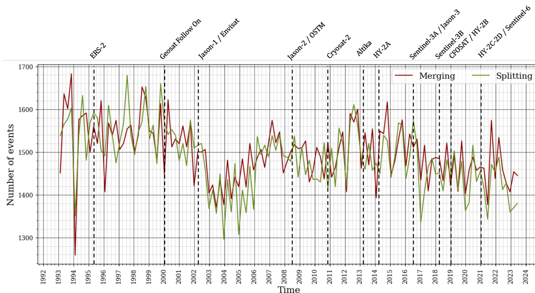
Figure 12. Temporal evolution of merging and splitting events.
