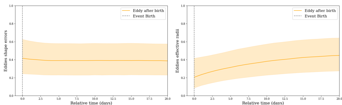
(a) Evolution of eddy shape errors around birth events. (b) Evolution of eddy effective radii around birth events.
