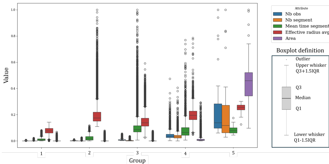
Figure 22. Box plots of the attributes for the five network clusters.
