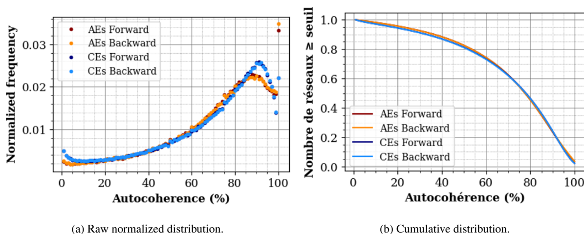
Figure 23. Raw and cumulative distributions of segment autocohérence scores.
