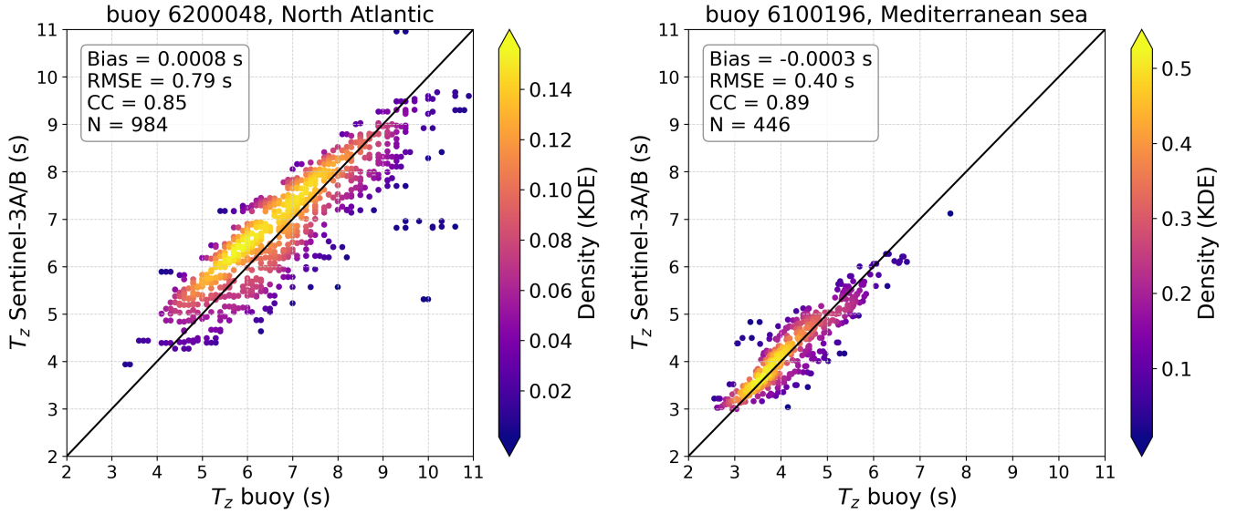
Figure 4. Scatter plots of wave period for the CMENS wave buoys 6200048 and 6100196, respectively, from Sentinel-3 A/B and the wave buoy at an Atlantic location (left) and a Mediterranean location (right).
