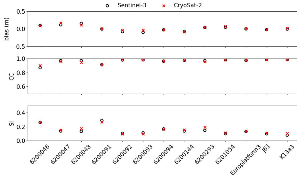
Figure 5. Comparison of statistical metrics for Hs. Red crosses – CryoSat-2, circles – Sentinel-3 A/Sentinel-3A/B. Region: British Isles.
