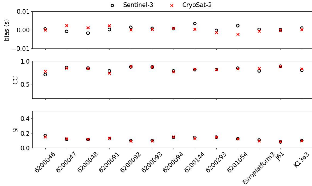
Figure 6. Comparison of statistical metrics for T_z . Red crosses – CryoSat-2, circles – Sentinel-3 A/Sentinel-3A/B. Region: British Isles.
