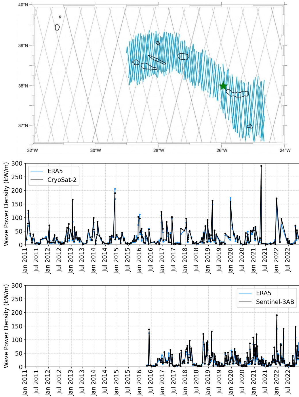
Figure 8. CryoSat-2 (blue) and Sentinel-3A/B (black) tracks in the Azores region for 2011. The time series location marked by an asterisk (top); comparison of the wave power density-derived time series from ERA5 and CryoSat-2 (middle) and comparison of the wave power density-derived time series from ERA5 and Sentinel-3A/B (bottom).
