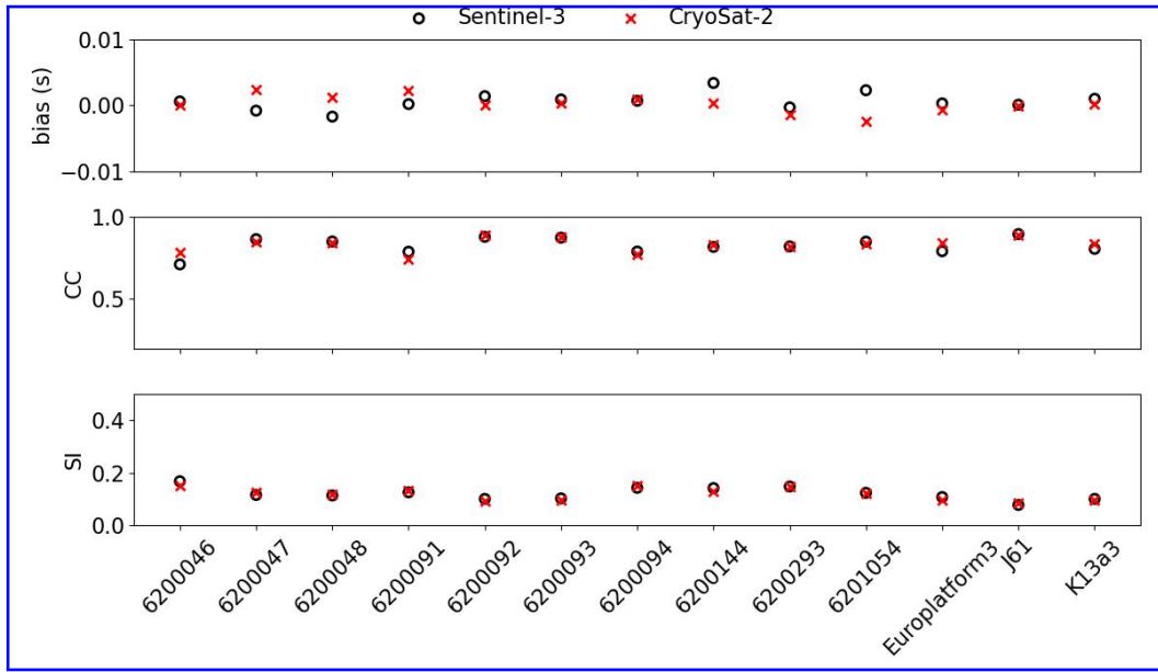
Figure 6. Comparison of statistical metrics for T_z . Red crosses – CryoSat-2, circles – Sentinel-3 A/B. Region: British Isles.
