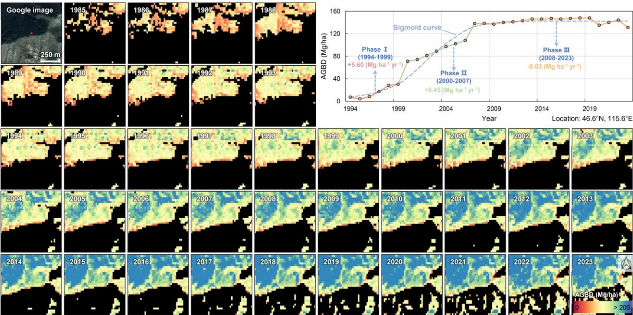
395 Figure 7: Temporal increase in AGBD of newly established forests under the Three-North Shelterbelt Program from 1985 to 2023, as captured by CFATD. (Satellite imagery: © Google Earth)
