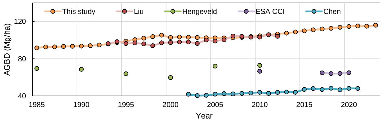
585 Figure 16: Comparative analysis of temporal dynamics across different AGB products.
