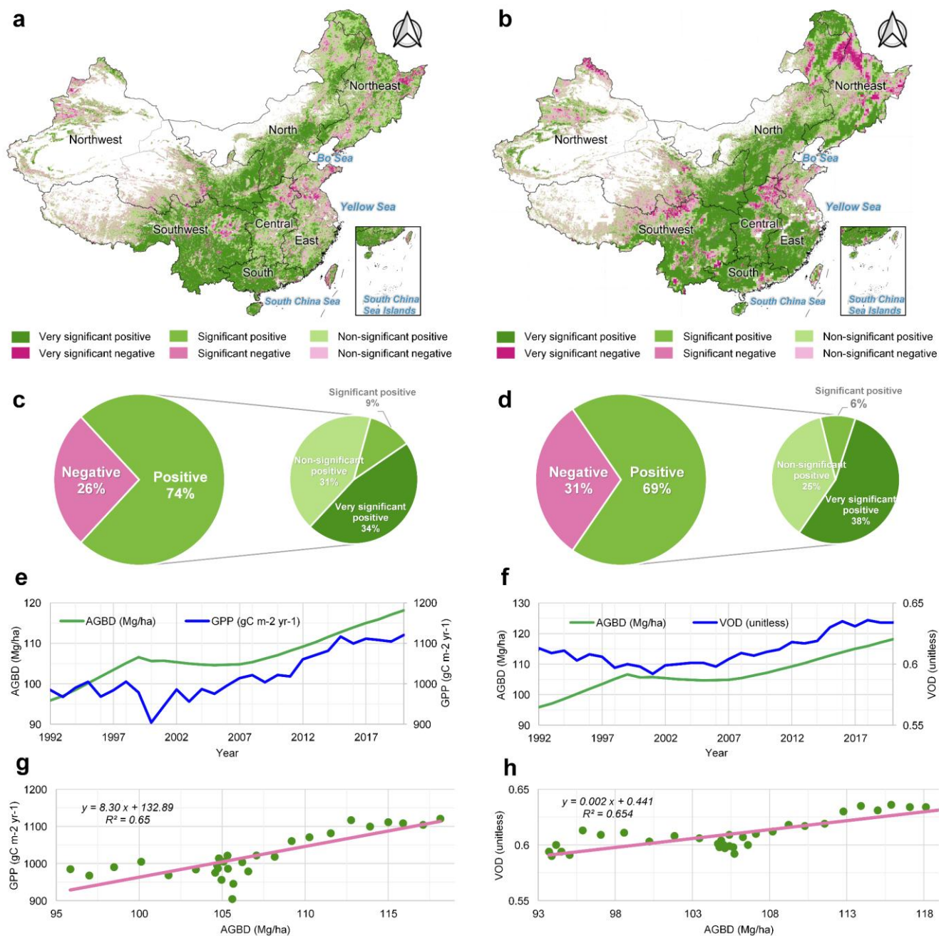
Figure 6: Cross-comparison of temporal dynamics between estimated AGBD and satellite-based datasets (GPP and VOD). (a, b) Pixel-level correlation maps between AGBD and GPP/VOD trends. (c–d) Fractions of highly significant ( p < 0.01 ), significant ( 0.01 \leq p < 0.05 ), and non-significant ( p \geq 0.05 ) pixels. (e, f) Temporal trajectories of national mean AGBD and GPP/VOD. (g–h) Relationships between national mean AGBD and GPP (1992–2020) or VOD (1987–2021).
