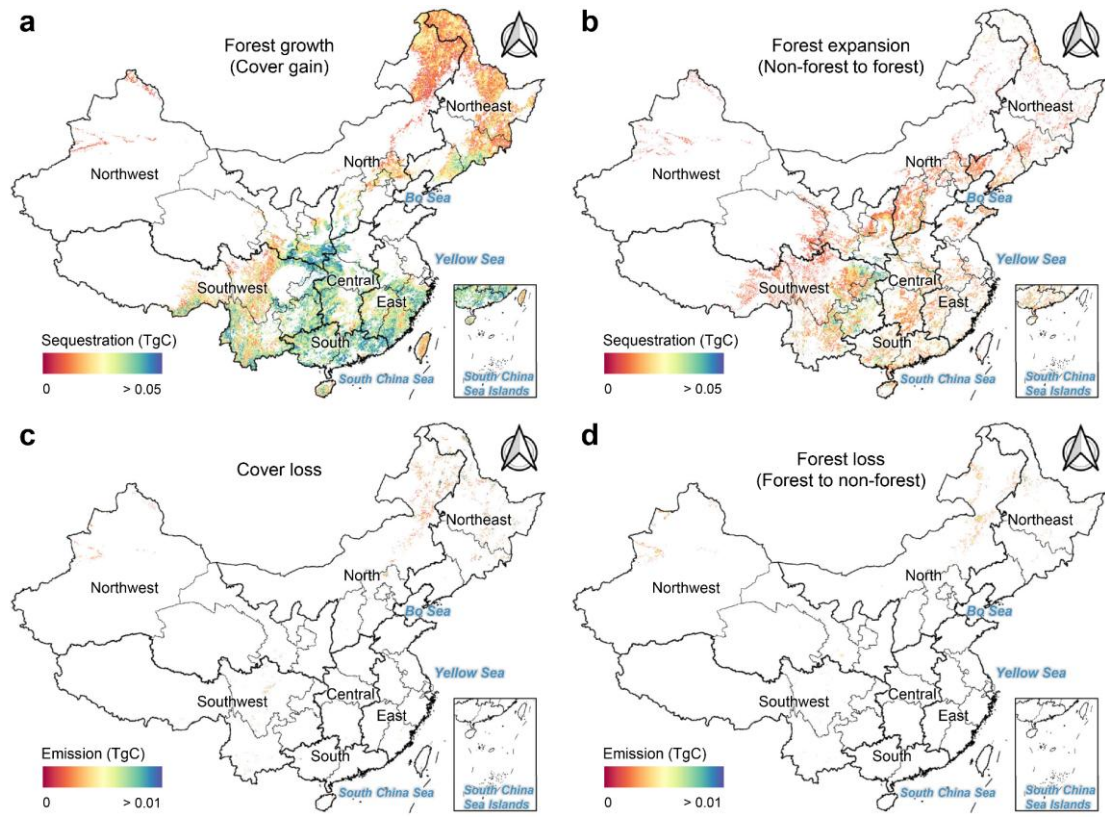
Figure 12: AGC Spatial changes induced by forest dynamics in China between 1985 and 2023. (a) and (b) represent the spatial distribution of carbon sequestration driven by forest growth and expansion, respectively. (c) and (d) illustrate the spatial distribution of carbon emissions resulting from tree cover loss and forest loss, respectively.
