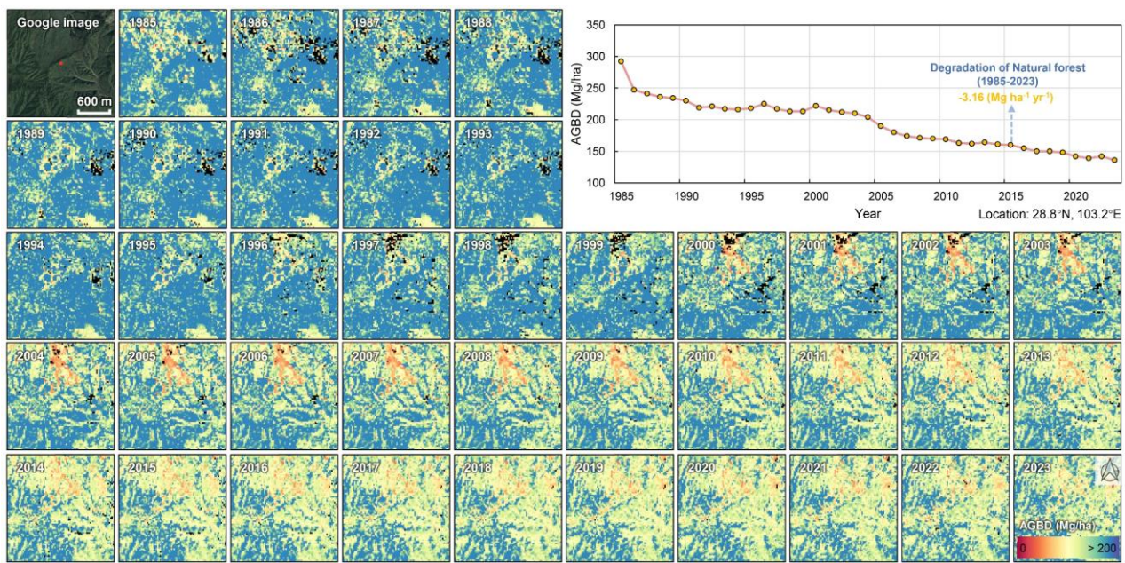
Figure 8: Temporal decline in AGBD of degraded natural forests in southwest China from 1985 to 2023, as captured by CFATD. (Satellite imagery: © Google Earth)
