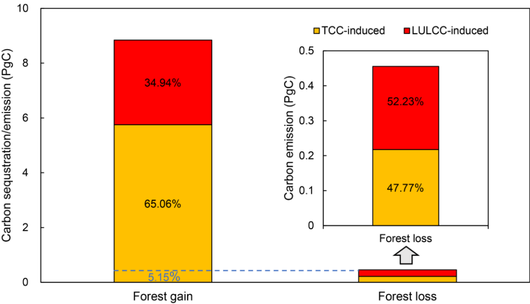
Figure 13: Quantification of AGC changes induced by forest dynamics in China between 1985 and 2023.
