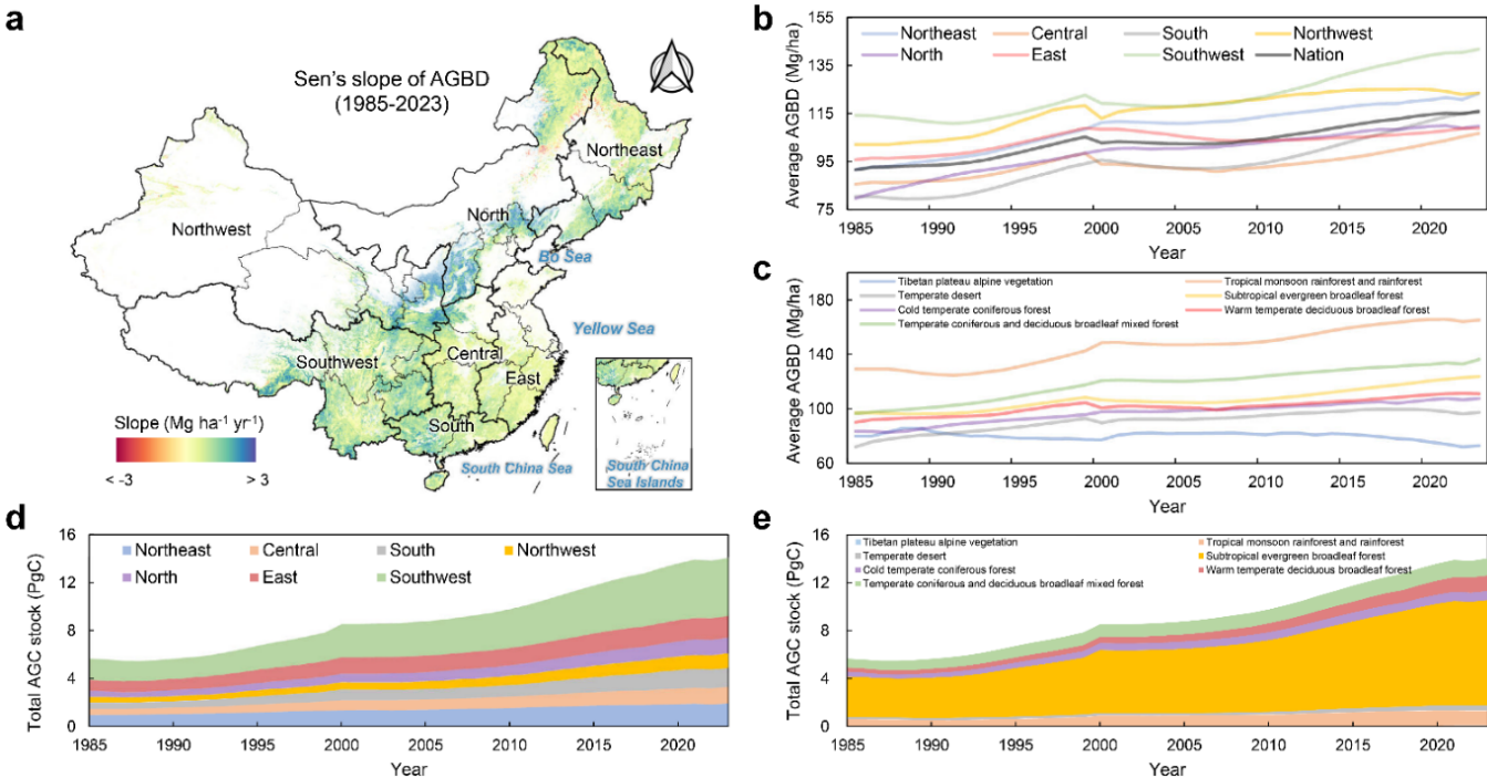
Figure 11: Long-term (1985–2023) trends in forest AGB and AGC stocks in China. (a) Pixel-level forest AGBD trend map derived from Sen’s slope analysis (Sen, 1968). (b) and (c) display annual changes in forest AGBD from 1985 to 2023 across geographical regions and ecoregions, respectively. (d) and (e) illustrate annual changes in total forest AGC stock over the same period, also across geographical regions and ecoregions. AGC is calculated from biomass using a conversion factor of 0.5.
