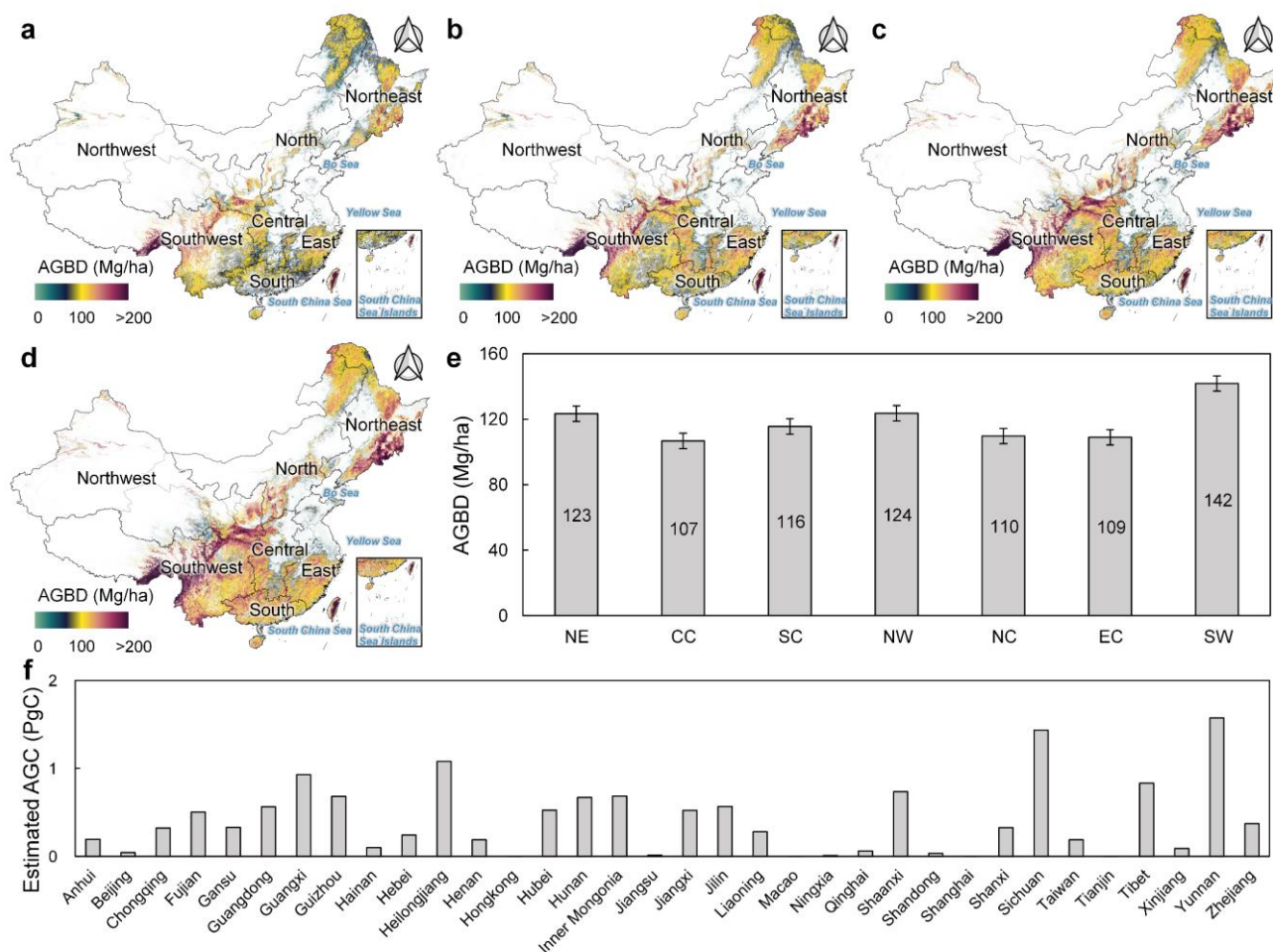
Figure 9: Spatial patterns of forest AGBD and regional summaries. (a–d) Spatial distribution of forest AGBD in China for 1985, 2000, 2015, and 2023, respectively. (e) Mean AGBD across different geographical regions. (f) Estimated forest AGC stock for different provinces.
