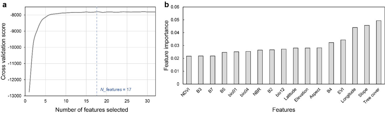
300 Figure. 2: Feature selection and importance analysis. (a) Cross-validation scores of the model with different numbers of features, measured by negative mean squared error. (b) Feature importance distribution based on Random Forest.
