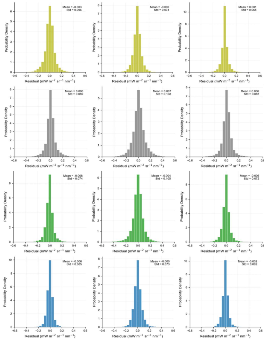
Figure S2 The Histograms of the downscaling residuals for GOME (1996, first row), SCIAMACHY (2008, second row), GOME-2 (2014, third row), and OCO-2 (2018, fourth row). The left, middle, and right columns correspond to results for January, July, and December, respectively.
