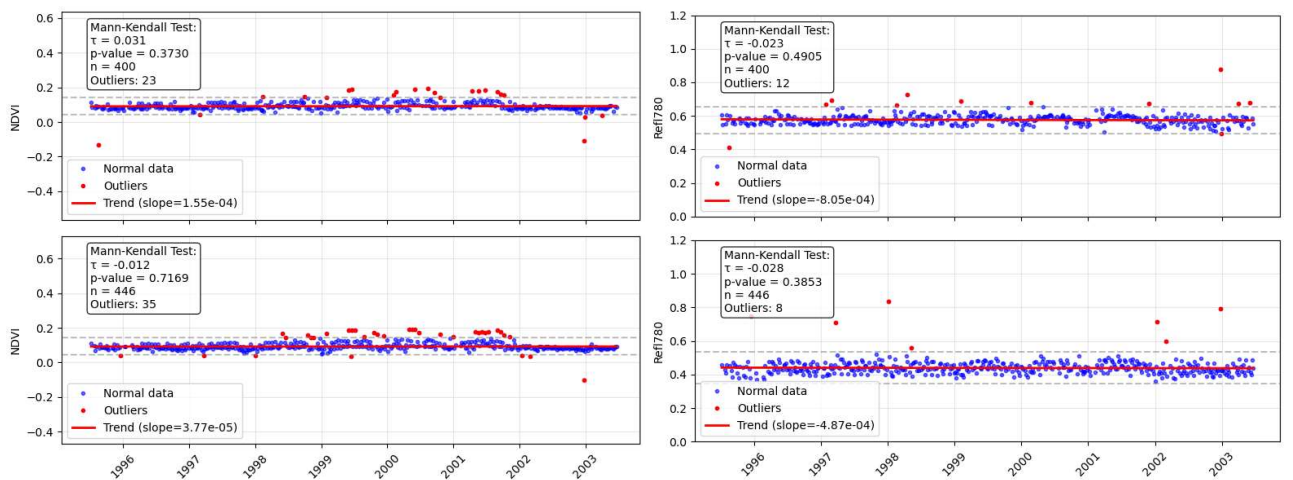
Figure R2 Long-term trends of GOME 780 nm reflectance and NDVI over the PICs.
