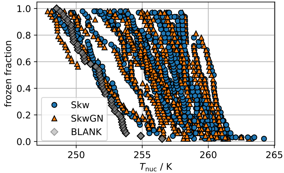
Figure 6. The frozen fraction as a function of the observed freezing temperature T_{\text{nuc}} for all filters, split into UAV (Skw), ground (SkwGN) and handling blank (BLANK) samples. Only one sample shows some diluted samples show a similar frozen fraction as the handling blank. Note that the handling blank suspension is very close to its Nanopure water background.
