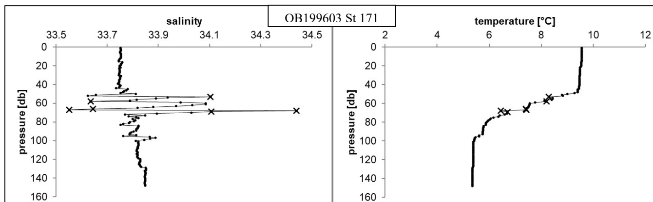
Figure 11. Quality control flags in a stratified profile
