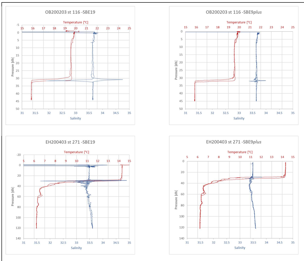
Figure 4: Temperature and salinity profiles versus pressure from different CTD models: SBE19 (left) vs SBE9plus (right). Solid lines indicate the downcast and dashed lines indicate the upcast.
