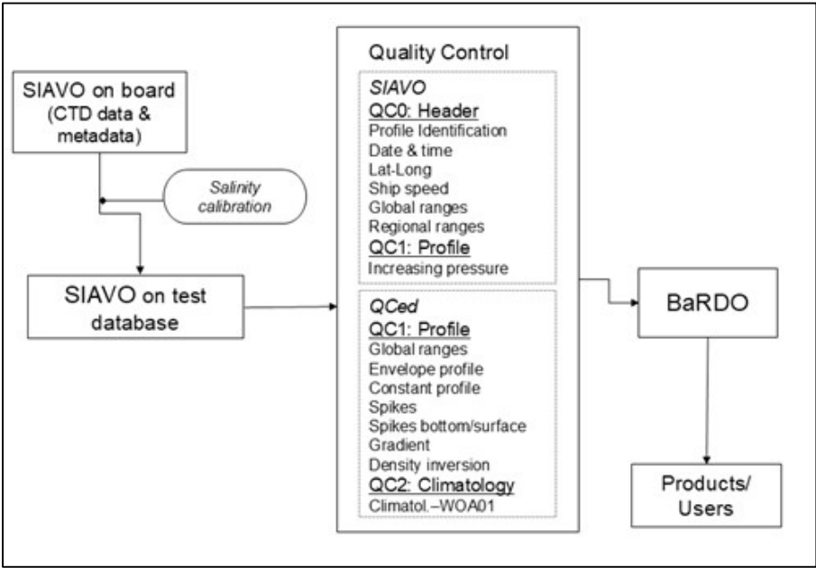
Figure 5: Data management system flow diagram
