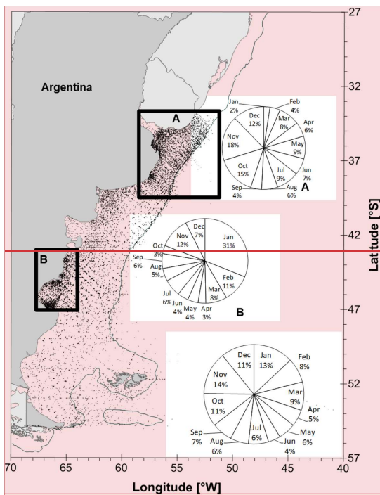
Figure 9: Geographical and monthly distribution of BaRDO stations.
