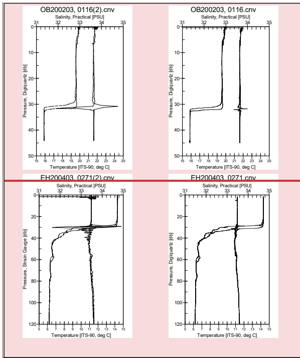
Figure 4: Temperature and salinity profiles versus pressure from different CTD models: SBE19 (left) vs SBE9plus (right). Solid lines indicate the downcast and dashed lines indicate the upcast.
