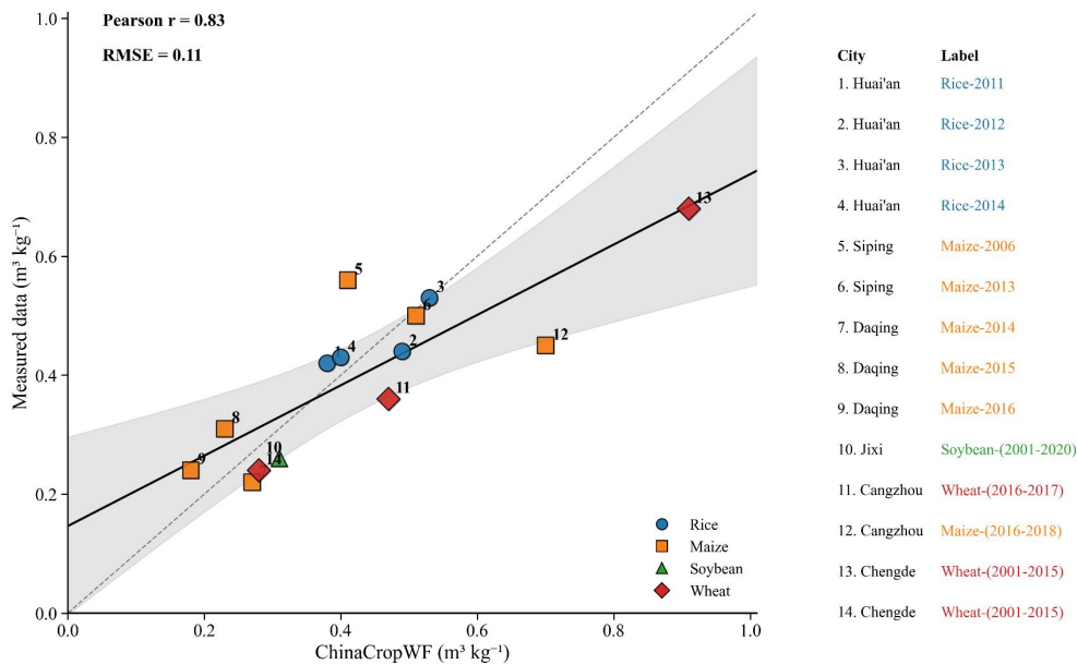
310 Figure 7: Comparison of ChinaCropWF with field-measured data.
