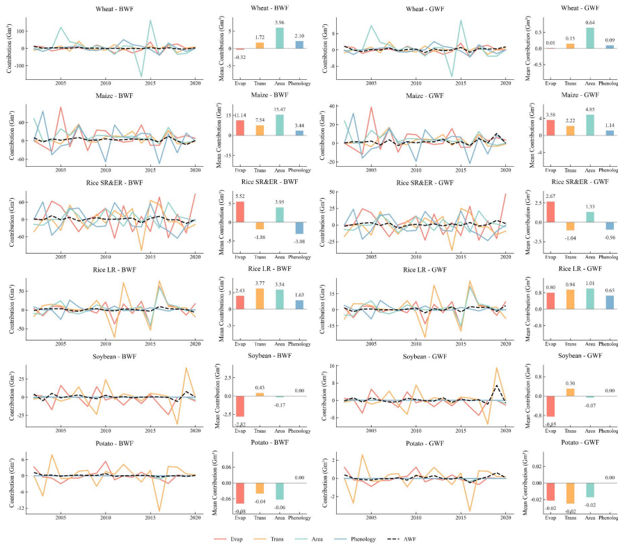
285 Figure 6: Evaluation of key driving factors of water footprint based on LMDI. The line charts illustrate the evolutionary trends driven by various factors over the period 2001-2020, while the bar charts present the multi-year average values attributed to each driving factor.
