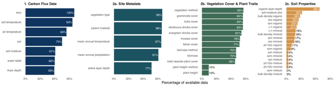
Figure 2. Data structure of the TundraFlux Database. Boxes represent the main data types: (1) Carbon flux data, including plot-level daily averages of ecosystem CO 2 respiration (R eco ) in g C-CO 2 m -2 d -1 and data measured along with flux measurements; (2) Metadata, including information on (a) site, (b) vegetation cover and plant traits at plot-level, and (c) Soil properties at plot level; and (3) Method data including documentation of experimental setups. Variables listed inside the boxes correspond to column names in the database (identical to Table S4).
