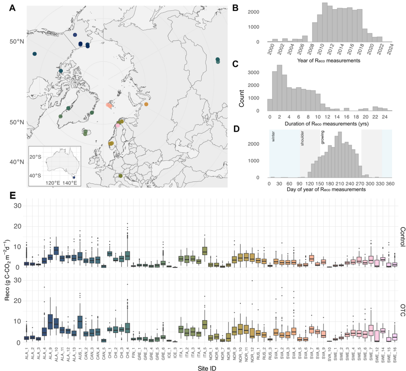
Figure 1 A. Map showing the locations of the 64 open-top chamber experiments from which the ecosystem CO 2 respiration (Reco) measurements in the TundraFlux Database were derived. Temporal spread of the data showing B. the distribution of the year of Reco measurements, C. the duration of Reco measurements (start of flux measurements - start of the experiment), and D. the distribution of day-of-year for Reco measurements, with shaded regions highlighting winter (Dec–Mar, light blue), shoulder (Oct–Nov, Apr–May, grey), and growing (Jun–Sep, white) seasons. E. Boxplots showing the daily average Reco (g C–CO 2 m -2 d -1 ) for each site, for both the unmanipulated control (i.e., ambient conditions, top) and the warmed treatment with open-top chambers (OTC, bottom). Boxes show the median and interquartile range (IQR, 25th–75th percentiles); whiskers extend to 1.5 × IQR, and values beyond the whiskers are plotted as outliers. Colours for Site_ID are the same for all panels. The database includes occasional negative and exact-zero Reco values. Negative values can result from instrument noise or brief net CO 2 uptake, while exact zeros may reflect contributor preprocessing (e.g., rounding or thresholding small fluxes).
