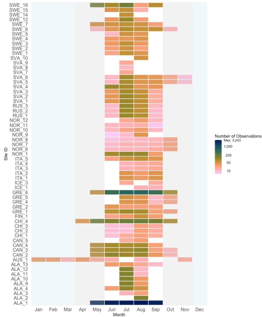
Figure 4. Monthly R_{eco} availability aggregated across all years. White/ light grey/ light blue cells = 0 observations. Color intensity based on \text{Log}_{10}(\text{Number of Observations} + 1) due to strong bias of ALA_1. Growing season = June–September in the Northern Hemisphere, December – March in the Southern Hemisphere. Except for AUS_1, shaded areas indicate winter months (light blue) and shoulder months (light grey).
