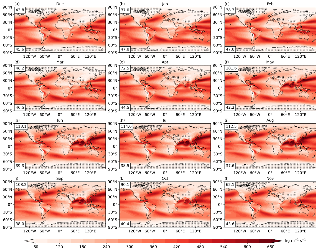
Figure 1. Climatological IVT threshold fields for each calendar month derived from during 1980–2019. Shadings indicate the final threshold values magnitude (units: \text{kg m}^{-1} \text{s}^{-1} ) obtained after combining the 85 th percentile value with the corresponding hemispheric lower limit. The lower limit values (units: \text{kg m}^{-1} \text{s}^{-1} ) for the Northern and Southern Hemispheres are annotated in the upper-left and lower-left, respectively. The dotted areas denote grids where the threshold is fixed at the hemispheric lower limit.
