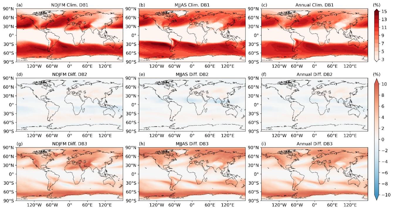
Figure 5. Global distribution of AR occurrence frequency using the present algorithm (DB1) for (a) the northern wintertime, (b) northern summertime, and (c) annual mean based on ERA5 during from 1980–2016. (d–i) As in (a–c) but for the frequency differences between DB1 and DB2 (d–f) and between DB1 and DB3 (g–i).
