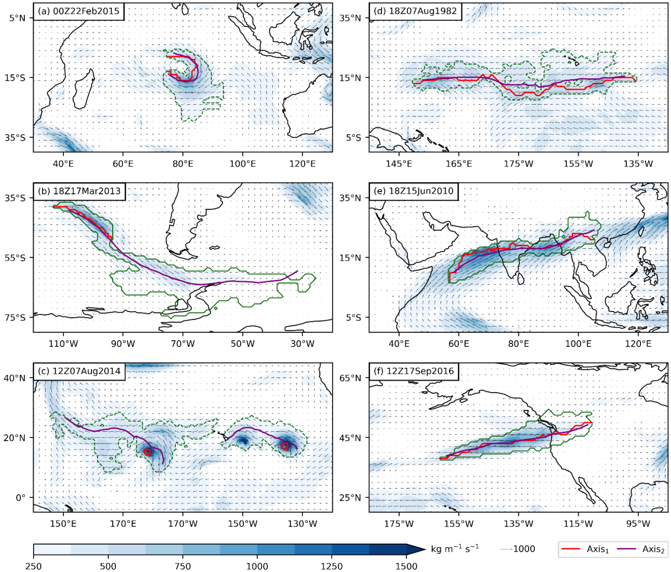
Figure 3. Examples of AR candidates. The shape boundaries of the candidates are marked by green curves; (solid green curves indicate identified AR activities, while dashed green curves indicate non-AR candidates, excluded by the algorithm). Axis 1 and Axis 2 are shown by solid red and purple curves, respectively. Shading indicates the IVT magnitude. The IVT is shown in vectors with the intensity shaded (units: \text{kg m}^{-1} \text{s}^{-1} ), and vectors denote the IVT direction.
