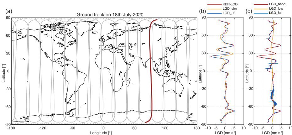
Figure 5: Examples of LGD data. (a) GRACE-FO ground tracks on 18 July 2020, with the red curve marking one ascending orbit selected for demonstration. Gray curves denote other satellite passes on the same day. (b) LGD values along the selected track in (a). The red, blue, and orange curves correspond to KBR-LGD, L2-based LGD, and climatology-based LGD, respectively (all from the KBR 325 dataset). (c) LGD from the LRI dataset, with blue, red, and orange curves representing full-spectrum, band-pass filtered, and low-frequency components, respectively.
