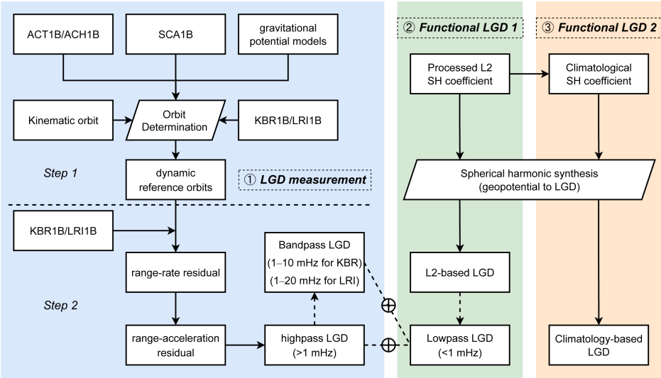
Figure 1: Workflow of LGD computation and required data inputs. The computation steps for LGD measurements, L2-based LGD, and climatology-based LGD are shown in blue, green, and yellow boxes, respectively. The workflow in terms of LGD measurements (blue boxes) is further divided into two sub-steps by a horizontal dashed line. Dashed arrows and lines indicate optional operations in terms of frequency spectrum (see details in Sect. 2.4). The mentioned ACT1B, ACH1B, SCA1B, KBR1B, and LRI1B data are collected from GRACE-FO L1B Release-04 dataset provided by Jet Propulsion Laboratory (JPL).
