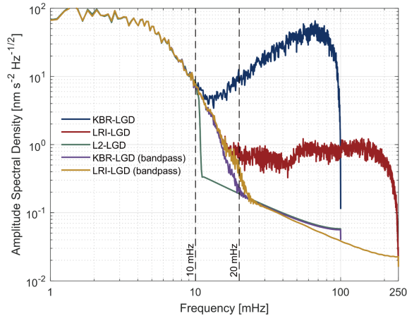
Figure 3: Amplitude spectral density of LGD time series on 18 July 2020. Blue and red curves represent LGD spectra derived from KBR and LRI observations, respectively. Green curve corresponds to LGD synthesized from L2 SH solutions. Purple and yellow curves show band-pass filtered LGD from KBR and LRI, with cutoff frequencies of 10 mHz and 20 mHz, respectively. Vertical dashed lines indicate the 10 mHz and 20 mHz thresholds used for filtering.
