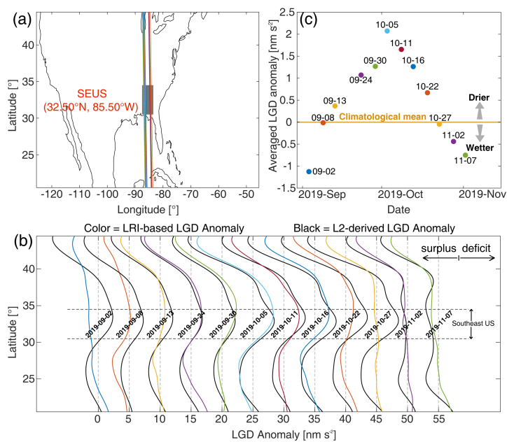
500 Figure 10: LGD analysis of the flash drought event in the SEUS from September to November 2019. (a) Study region (gray box) centered at 32.5° N, 85.5° W. Colored lines represent GRACE-FO ground tracks intersecting the region during September–early November. (b) Along-track LGD anomalies for each satellite pass, with colored lines denoting LRI-based anomalies (LRI-LGD minus climatological LGD) and black lines showing L2-derived anomalies (LGD L2 minus climatological LGD) for comparison. Negative LGD anomalies indicate wetter-than-normal conditions, while positive anomalies indicate drier-than-normal conditions. (c) Averaged LGD anomalies over the SEUS through weighted averaging.
