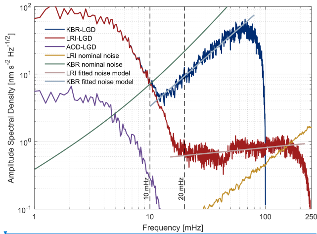
Figure 12: Amplitude spectral density of intersatellite ranging measurements, instrument noise, and background model errors, all expressed in terms of line-of-sight gravity differences. Green and yellow curves denote the nominal instrument noise from the KBR and LRI ranging systems, respectively. Blue and red curves show the spectra of KBR-LGD and LRI-LGD measurements. The purple curve represents errors associated with background model differences (AOD1B RL07 vs. RL06). The light blue and light red curves show the
