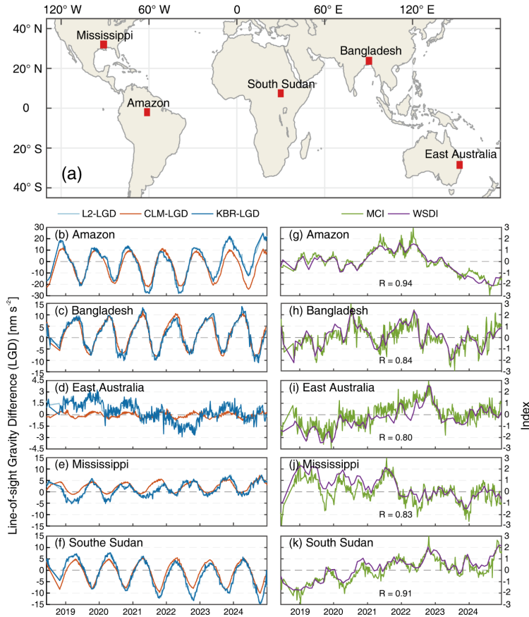
535 Figure 11: Identification and characterization of sub-monthly hydrological extremes in global hotspot regions during the GRACE-FO period using the Mass Change Index (MCI). (a) Locations of the five hotspot regions (red boxes): Mississippi, Amazon, South Sudan, Bangladesh, and eastern Australia. (b–f) Regional LGD time series, including measured LGD (dark blue lines), synthetic LGD_L2 (light blue lines), and climatology-based LGD (orange lines). Note that panels (b) and (d) use a different y-axis scale. (g–k) Comparison of the MCI (green lines) with the Water Storage Deficit Index (WSDI; purple lines) derived from monthly L2-derived TWS. Correlation coefficients (R) between WSDI and MCI are given in each panel. 540
