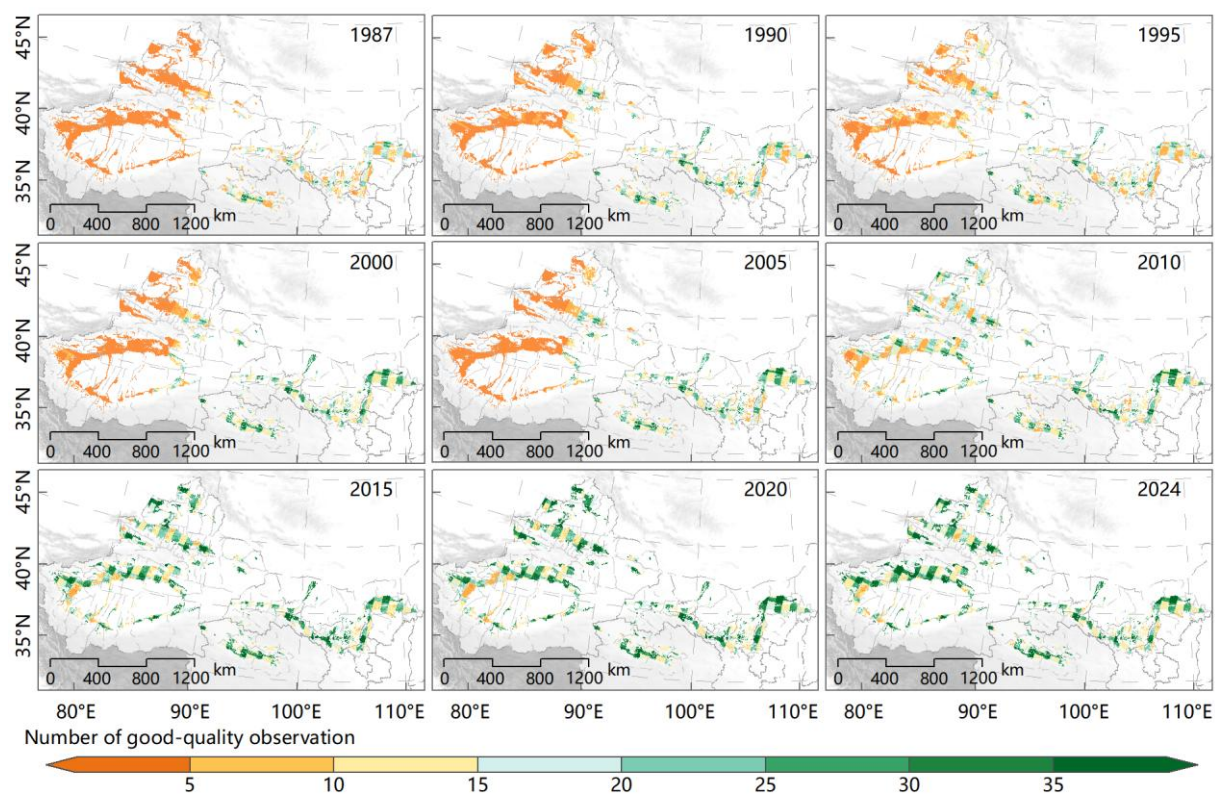
Figure S6. Spatial distribution of good-quality observations of Landsat data in China's oases.
