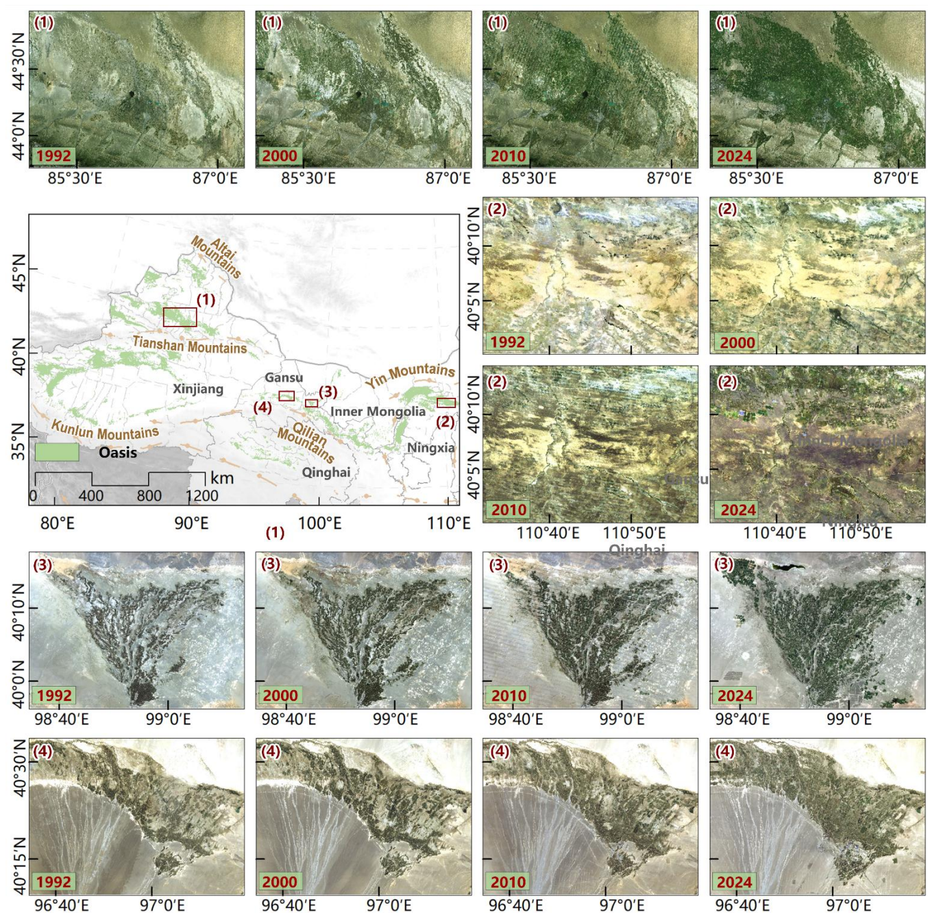
Figure S4. The Expansion Process of China's Oases. All the Landsat images are freely provided by USGS.
