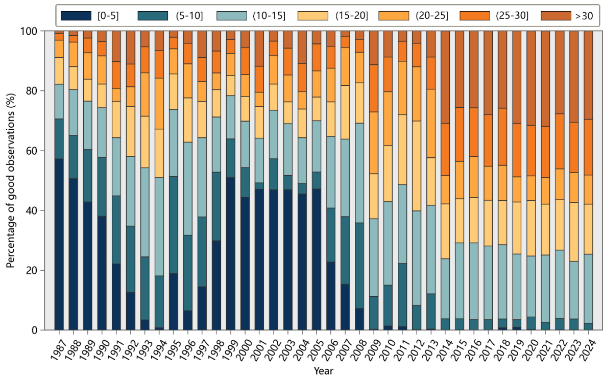
Figure S5. Percentage of good-quality observations during 1987–2024. Different colors indicate the number of Landsat images.
