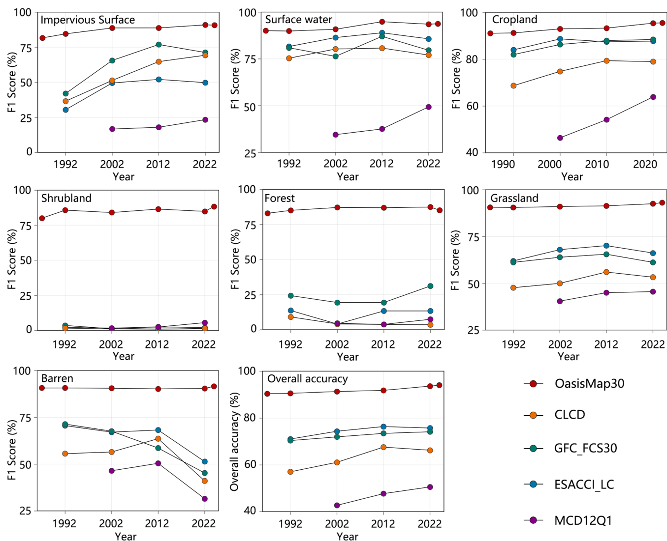
Figure S1. F1 score and overall accuracy for CLCD, GLC_FCS30, ESACCI_LC, MCD12Q1 and OasisMap30 based on visually interpreted test samples.
