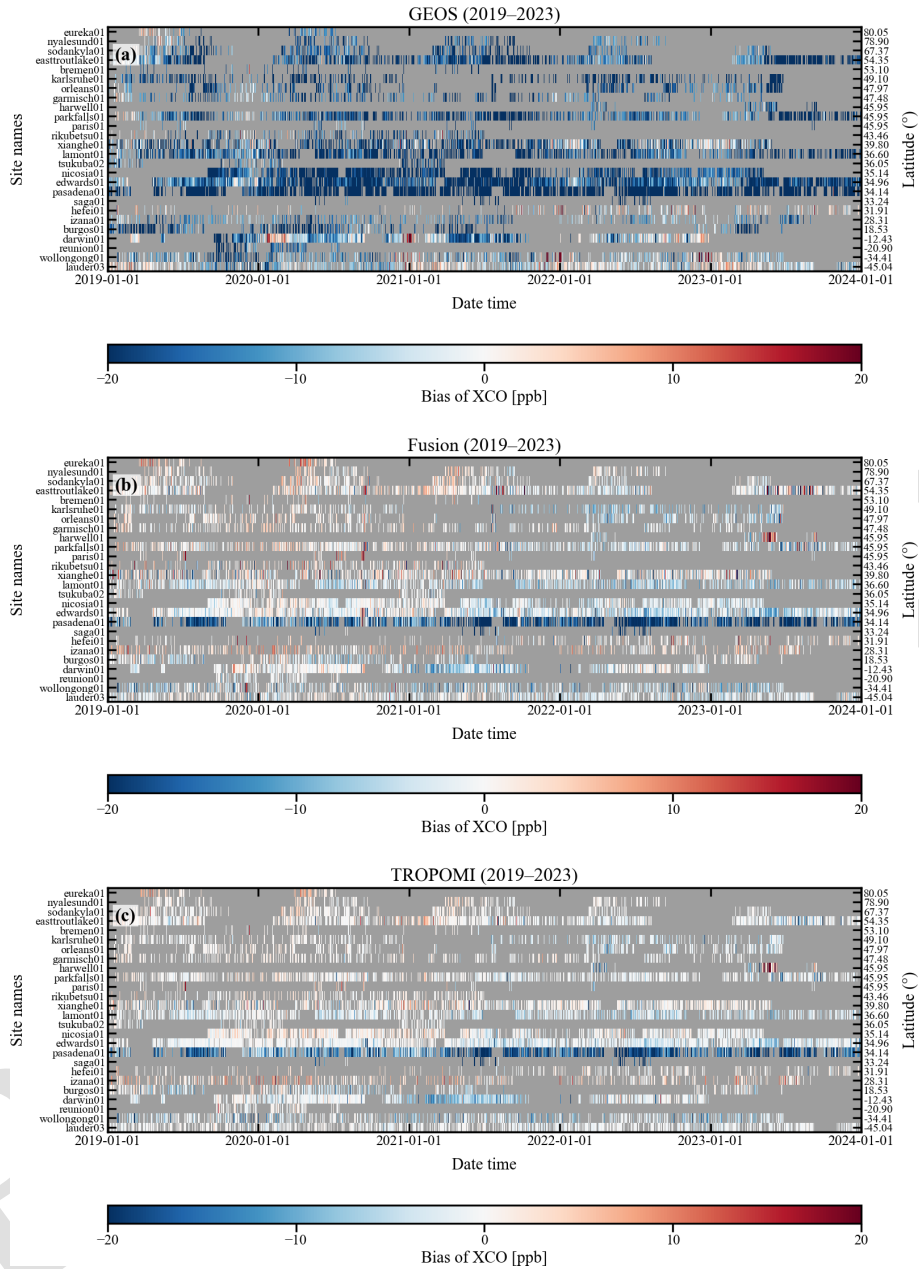
Figure 10. Heat maps of the biases between daily (a) GEOS, (b) fused, and (c) TROPOMI XCO and TCCON XCO over time and latitude. Color ramps stand for the biases of XCO. Background colors (grey) indicate the missing data.
