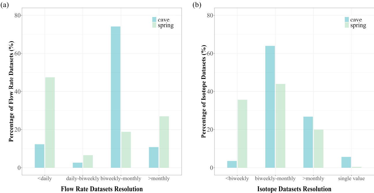
343 Figure 6: (a) Proportions of temporal resolution categories of discharge and drip rate datasets for karst springs and cave drip sites; The 344 datasets are divided into four resolution levels: finer than daily , daily to biweekly , biweekly to monthly and coarser than monthly . (b) 345 Proportions of temporal resolution categories of stable isotopes for karst springs and caves. The resolutions are stratified into four categories: 346 finer than biweekly , biweekly to monthly , coarser than monthly and single-value records . 347
