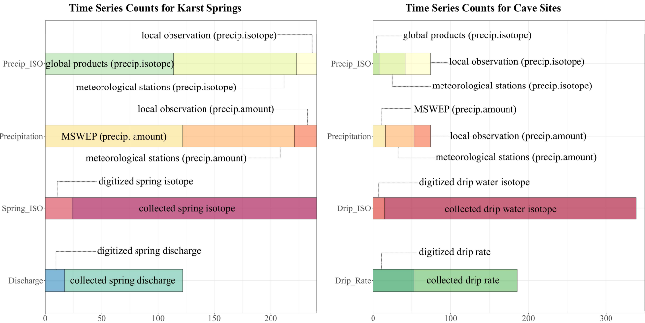
239 Figure 2: Distribution of time series counts for hydrological and isotopic datasets in WoKaS-Iso database, categorized by source types. For 240 karst springs, precipitation isotopes come from local observations (18), meteorological stations (109), and global model products (114), 241 while precipitation amounts come from local observations (20), meteorological stations (99), and MSWEP (122). Spring water isotopes 242 include collected (217) and digitized (24) data, and spring discharge includes collected (105) and digitized (17) data. For caves, precipitation 243 isotopes come from local observations (33), meteorological stations (33), and global model products (8). Cave drip water isotopes include 244 collected (324) and digitized (15) data, and cave drip rates include collected (133) and digitized (53) data.
