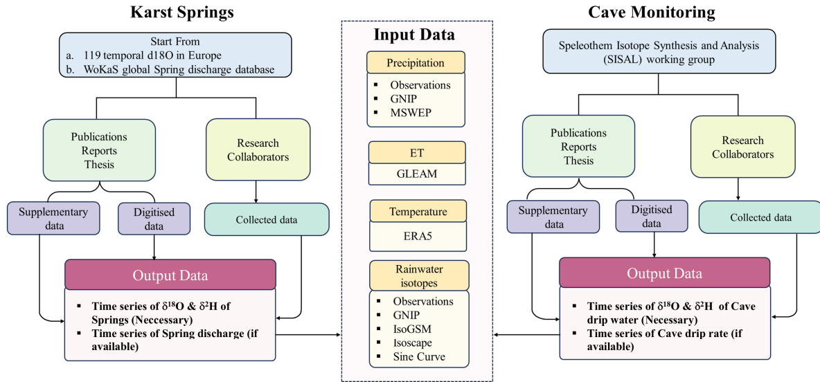
200 201 Figure 1: Workflow of the karst spring and cave drip water stable isotopes database construction. The left branch illustrates the karst spring 202 component, built upon the WoKaS global spring discharge database and an initial European stable isotope compilation (Hartmann et al., 203 2021), with data sourced from publications, reports, theses, and research collaborators via collection and digitization. The right branch shows
