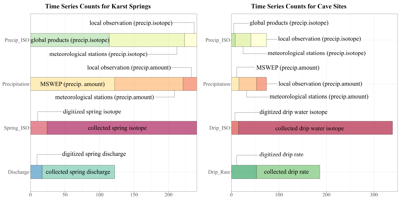
242 Figure 2: Distribution of time series counts for hydrological and isotopic datasets in the WoKaS-Iso database, categorized by source types. 243 For karst springs, precipitation isotopes come from local observations (18), meteorological stations (109), and global model products (114), 244 while precipitation amounts come from local observations (20), meteorological stations (99), and MSWEP (122). Spring water isotopes 245 include collected (217) and digitized (24) data, and spring discharge includes collected (105) and digitized (17) data. For caves, precipitation 246 isotopes come from local observations (33), meteorological stations (33), and global model products (8). Cave drip water isotopes include 247 collected (324) and digitized (15) data, and cave drip rates include collected (133) and digitized (53) data. 248
