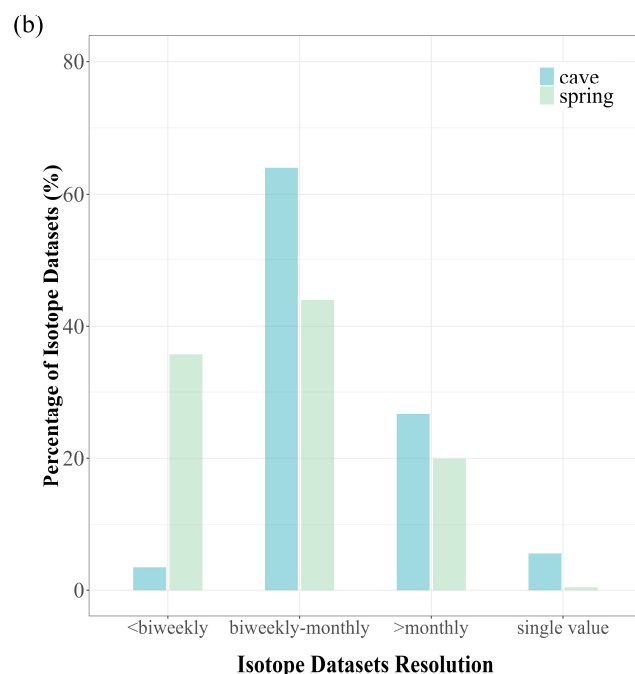
Figure 65: (a) Proportions of temporal resolution categories of discharge and drip rate datasets for karst springs and cave drip sites; The datasets are divided into four resolution levels: finer than daily , daily to biweekly , biweekly to monthly and coarser than monthly . (b)
