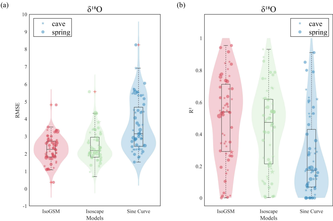
Figure 76: Statistical comparison of three model performance for \delta^{18}\text{O} in precipitation at cave (stars) and springs sites (circles). (a) Root Mean Square Error (RMSE); (b) Coefficient of determination ( R^2 ). Violin plots show the distribution of performance metrics for each model: IsoGSM (red), Isoscape (green), and Sine Curve (blue). Boxplots within violin indicate the median, interquartile range and outliers. Lower RMSE and higher R^2 indicate better model performance.
