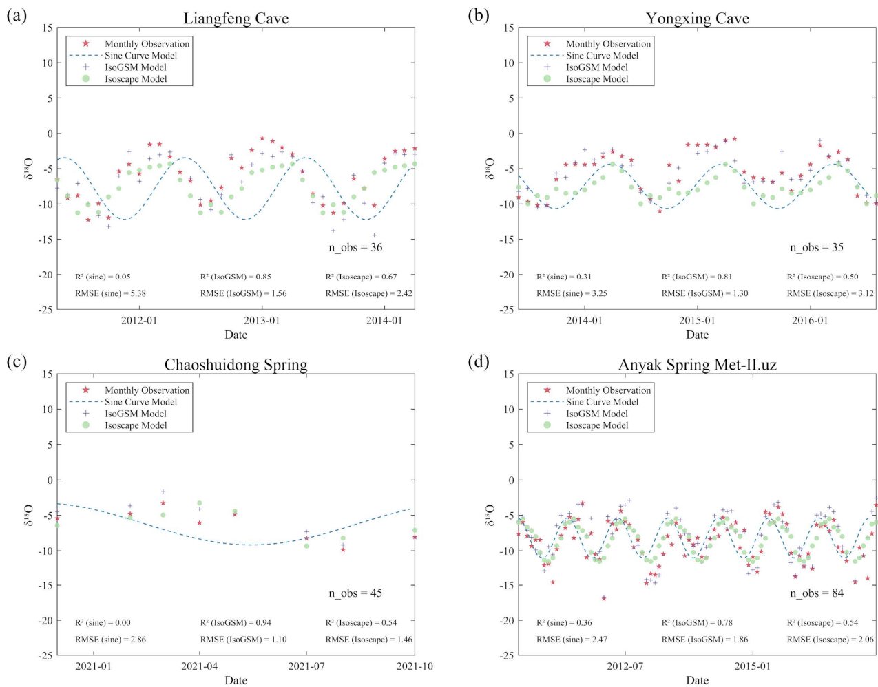
Figure 97: Time series comparison of modelled and observed monthly \delta^{18}\text{O} in precipitation at two cave sites (a–b) and two spring sites (c–d). Observations (red stars) are compared with estimates from the Sine Curve model (dashed blue line), IsoGSM (purple crosses), and the Isoscape model (green circles). Each panel shows the number of monthly observations (n.obs) and model performance statistics (R 2 and RMSE).
