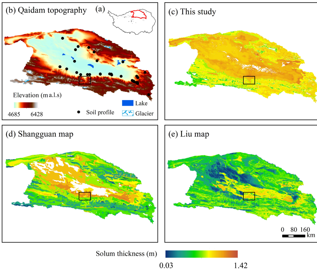
Fig. 7 Comparison of solum thickness datasets in the Qaidam Basin. (b) Topography of the basin with an inset (a) showing its location on the QTP. Spatial distribution of solum thickness simulated by (c) this study, (d) the Shangguan map, and (e) the Liu map. The black box highlights the topographic gap in the southern mountain rim discussed in the text. White patches represent no data.
