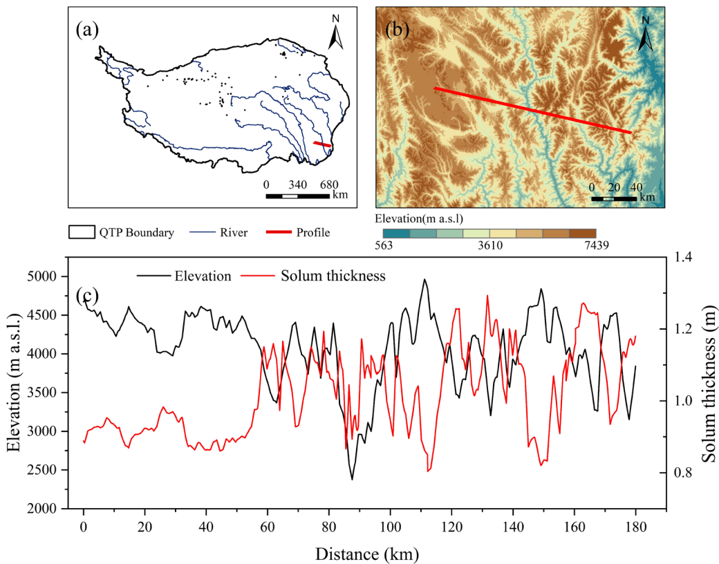
Fig. 5 Topographic controls on solum thickness along a transect in the Hengduan Mountains. (a) Location of the study transect on the southeastern QTP. (b) Local topography of the transect area. (c) Cross-sectional profile illustrating the inverse relationship between elevation (black line) and simulated solum thickness (red line), where thickness peaks in valley floors and minimizes on ridge crests.
