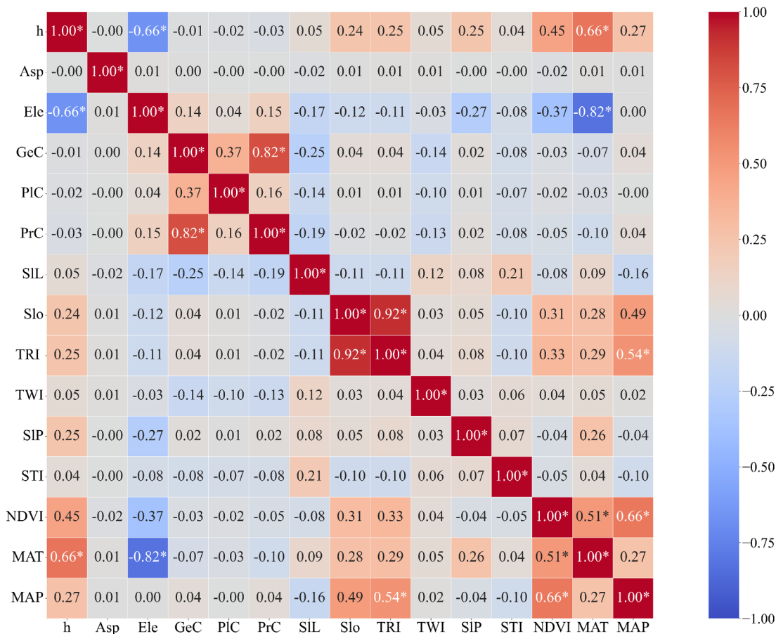
Fig. 4 Pearson correlation matrix between simulated solum thickness ( h ) and environmental variables. Red represents positive correlations and blue represents negative correlations. Asterisks denote statistically significant correlations ( p < 0.05 ). Refer to Table 1
