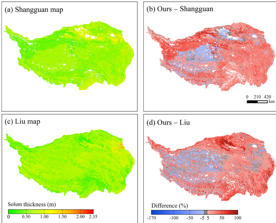
Fig. 6 Comparison of solum thickness datasets across the QTP. Spatial distribution of solum thickness derived from (a) the Shangguan map and (c) the Liu map. Relative percentage difference between the simulated results of this study and (b) the Shangguan map and (d) the Liu map. Positive values indicate that our model predicts thicker solum than the reference datasets, while negative values indicate thinner solum. White patches represent null values (no data). In the Shangguan map, these correspond to defined non-soil units, while in our study, these correspond to masked glaciers and lakes.
