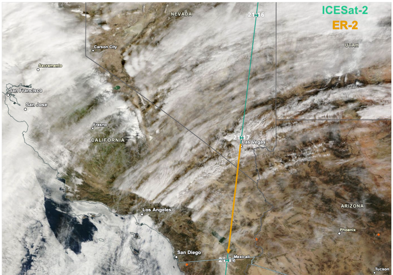
690 Figure 3: An example of the targeted satellite track (green, ICESat-2) and the roughly 30-minute long ER-2 underflight segment (orange) on 03 February 2025. The satellite and aircraft tracks are overlaid on the True Color Corrected Reflectance from MODIS on the Terra satellite, which shows optically thin cirrus clouds over southern California.
