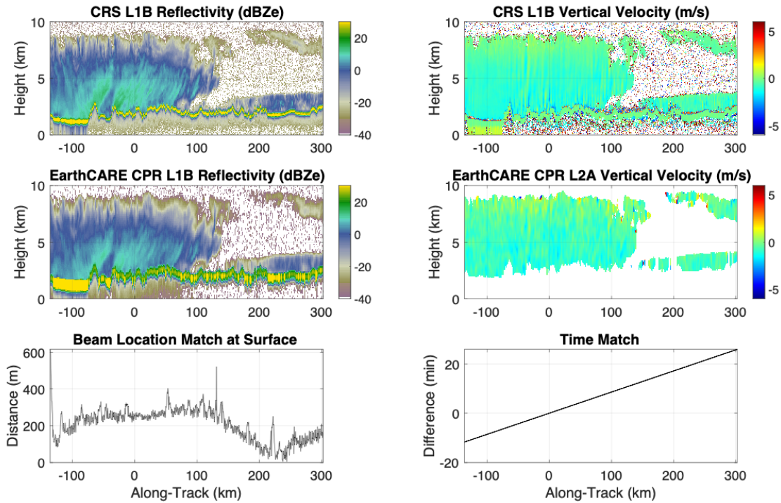
Figure 6: The 94 GHz reflectivity (left) and Doppler velocity (right) for CRS (top panels) and EarthCARE CPR BA baseline (middle panels) that show large and precipitating hydrometeors as the ER-2 flew over northern Utah on 20 February 2025 (track in red, Figure 4). The bottom panels show the time match between the aircraft and EarthCARE satellite.
