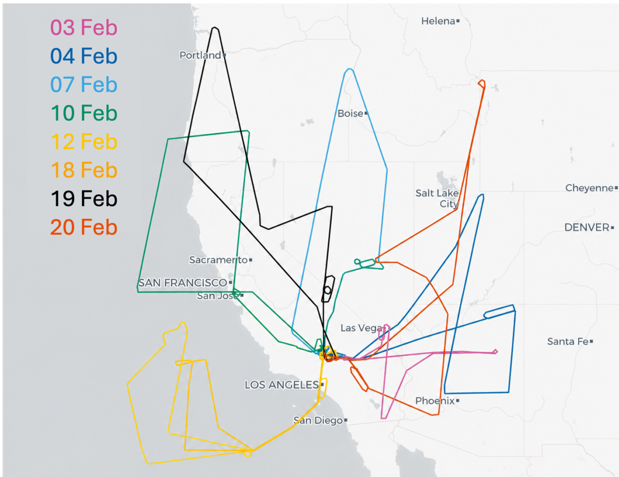
695 Figure 4: Flight tracks for the GLOVE field campaign. Eight flights were conducted from 3–20 February 2025 over California, Nevada, Arizona, Oregon, Utah, Idaho, and the coastal Pacific Ocean from the Armstrong Flight Research Center in Edwards, California.
