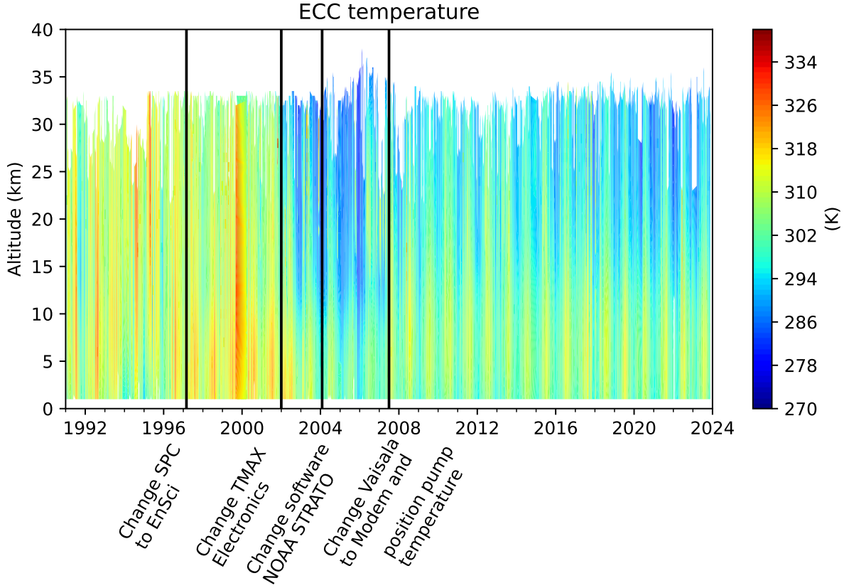
Figure 4. Time evolution of the ozonesonde homogenized internal pump temperature in K as a function of altitude. Major changes of the ECC instrument are shown in the bottom part of the figure.
