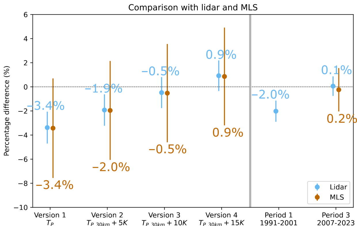
Figure 9. Evaluation of ECC ozone concentration compared with lidar and MLS ozone concentrations. Results are presented as medians and 2*standard errors of percentage difference for a corrected and two uncorrected periods. An uncorrected and three corrected ECC ozone concentrations are tested for the period January 2002–June 2007.
