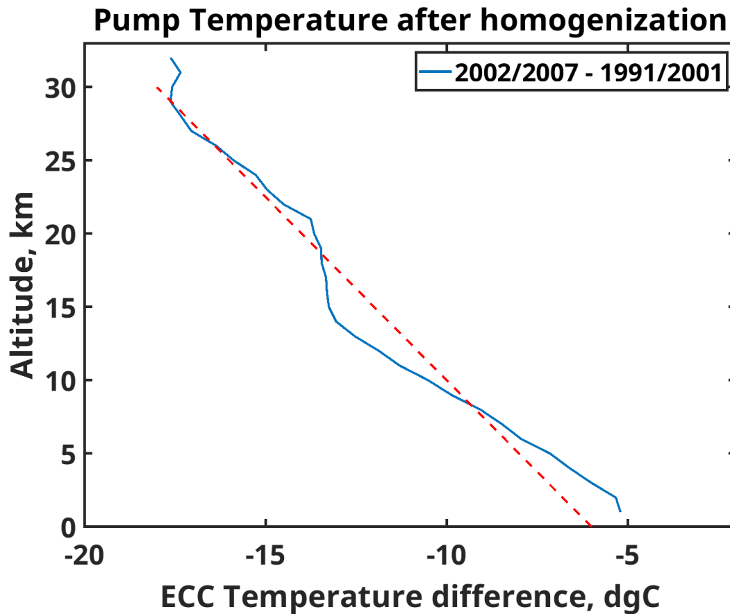
Figure 7. Vertical profile of the mean homogenized ECC pump temperature difference in K between period 2002/2007 and period 1991/2001. The red dotted line shows a linear altitude-dependent correction with an increasing rate of 0.4 K/km.
