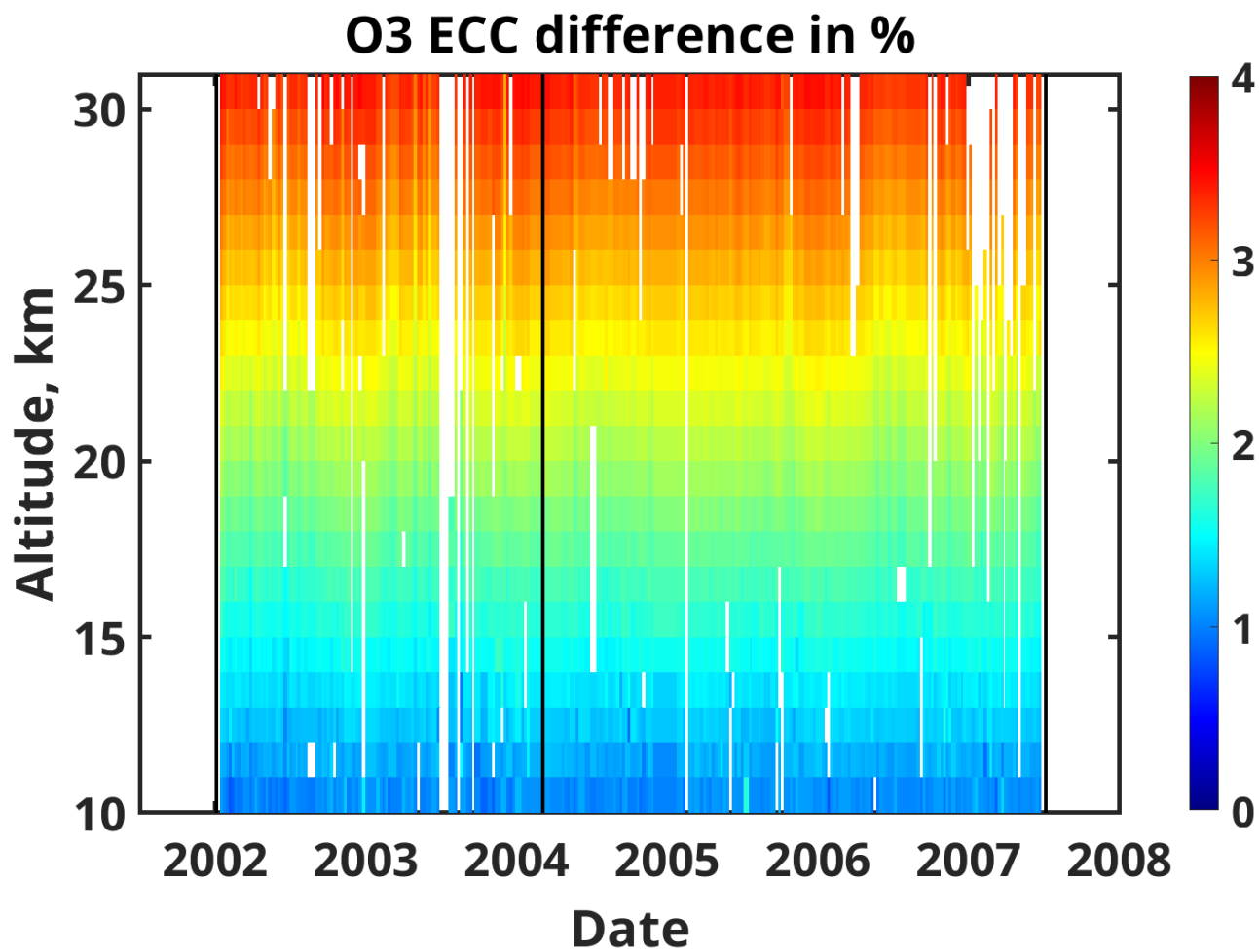
Figure 10. Differences between the ozone concentration calculated without any correction of the homogenized ECC temperature (Version 1 of T_{P_{cor}} ) and with Version 3 of T_{P_{cor}} as a function of altitude for the time period 2002-2007.
