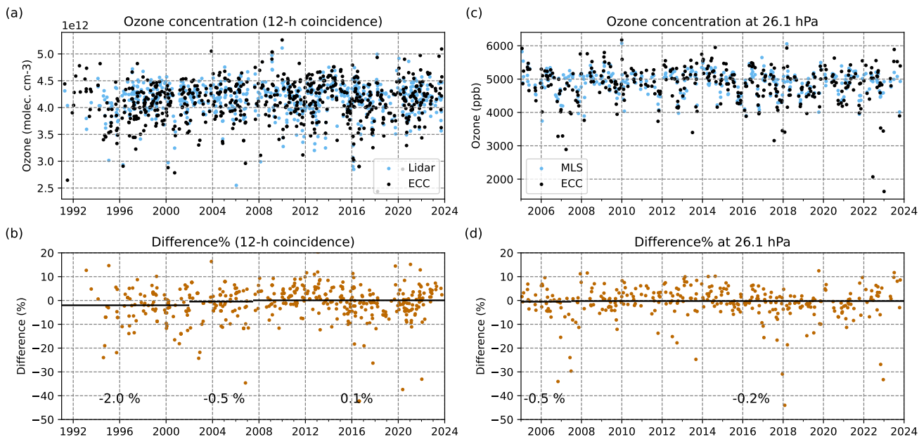
Figure 12. Time series of ozone concentration of the stratospheric lidar and the ECC ozonesonde at 25 km, and MLS and the ECC ozonesonde at 26.1 hPa (a and c). Ozone concentration and (b and d) relative ECC minus lidar ozone concentration differences for the coincident (< 12 h) profiles. Ozone concentrations for (a–b) are calculated at altitude 25 km by averaging ozone over a range of \pm 1 km. Ozone concentrations for (c–d) are calculated at pressure level 26.1 hPa by averaging ozone over a range of \pm 1 layer (31.6 hPa–21.5 hPa). Black lines with values in (b and d) indicate average relative differences for the periods same as Fig. 1-2.
