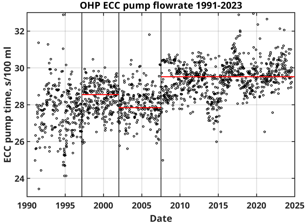
Figure 3. Time evolution of the ozonesonde time in s for pumping 100 ml. The black vertical bar correspond to changes in sondes type or processing software (see Fig. 4). The horizontal red lines are the median values of the pumping time used in Fig.6, Table 1, 2.
