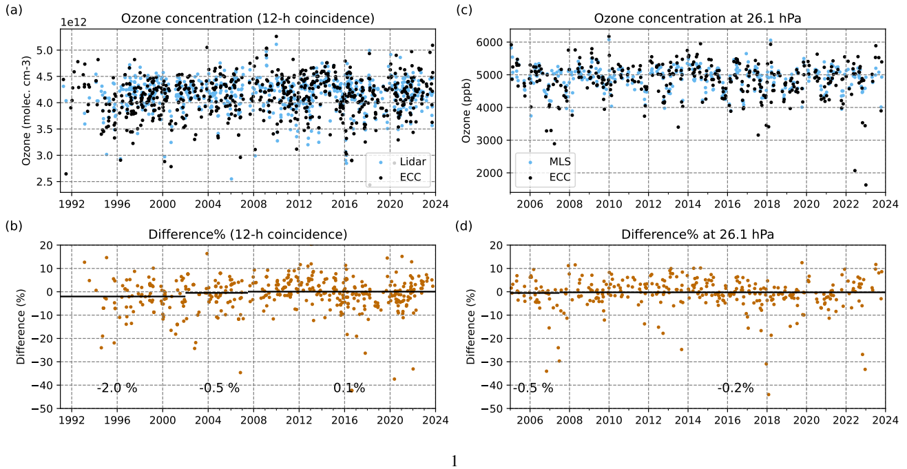
Figure 12. Time series of ozone concentration of the stratospheric lidar and the ECC ozonesonde at 25 km, and MLS and the ECC ozonesonde at 26.1 hPa (a and c). Ozone concentration and (b and d) relative ECC minus lidar ozone concentration differences for the coincident (< 12 h) profiles. Ozone concentrations for (a–b) are calculated at altitude 25 km by averaging ozone over a range of \pm 1 km. Ozone concentrations for (c–d) are calculated at pressure level 26.1 hPa by averaging ozone over a range of \pm 1 layer (31.6 hPa–21.5 hPa). Black lines with values in (b and d) indicate average relative differences for the periods same as Fig. 1-2.
