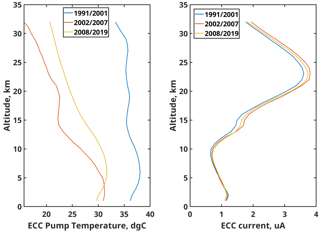
Figure 5. Mean vertical profile of homogenized ECC pump temperature in ^{\circ}\text{C} (left panel) and ECC current in \mu\text{A} (right panel) for period 1991/2001, 2002/2007 and 2008/2019.
