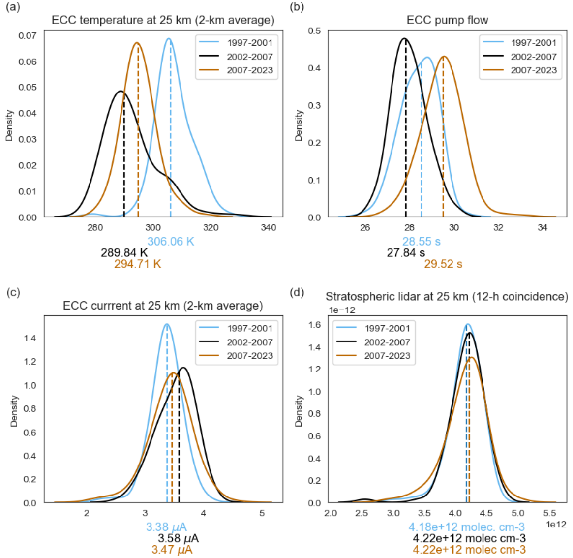
Figure 6. Density plot of the key factors in calculating the ozone partial pressure. (a) ECC homogenized temperature T_P at 25 km in K , (b) ECC pumping time for 100 ml in s , (c) ECC current at 25 km in \mu\text{A} , and (d) ozone concentration in \text{molecule.cm}^{-3} measured by the stratospheric lidar at OHP for three periods: March 1997–December 2001 (light blue), January 2002–June 2007 (black) and July 2007–December 2023 (brown). The dashed lines and values in the bottom part of figures show medians summarized in Table 1.
