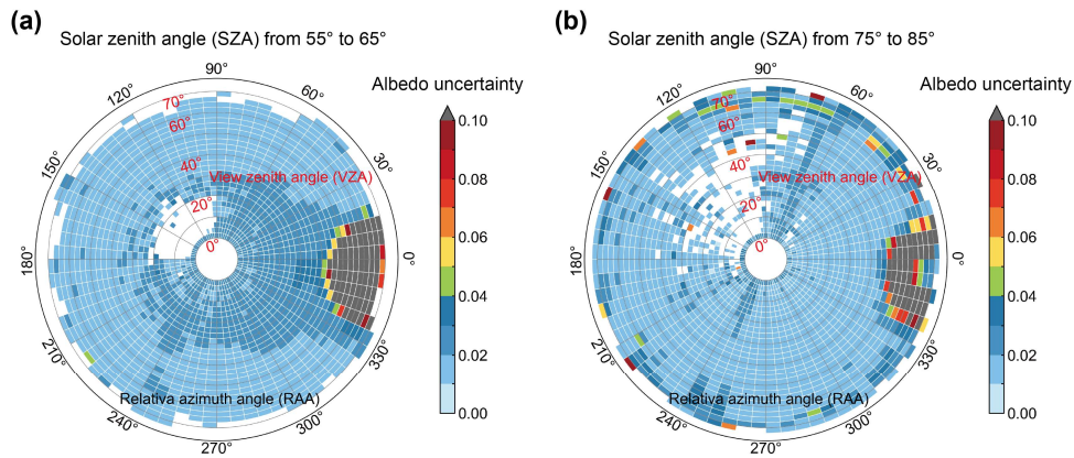
Figure 5. Angular distribution of the mean uncertainty in sea ice albedo retrieval. (a) Solar zenith angle from 55° to 65°; (b) Solar zenith angle from 75° to 85°. In the polar coordinate system, the radial direction
