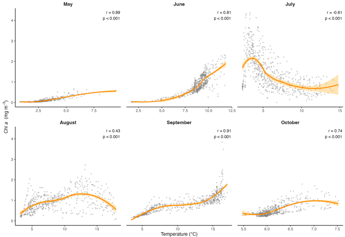
Figure A1: Scatter plots showing the monthly relationships between Chl a and temperature, across the transect. The orange line
