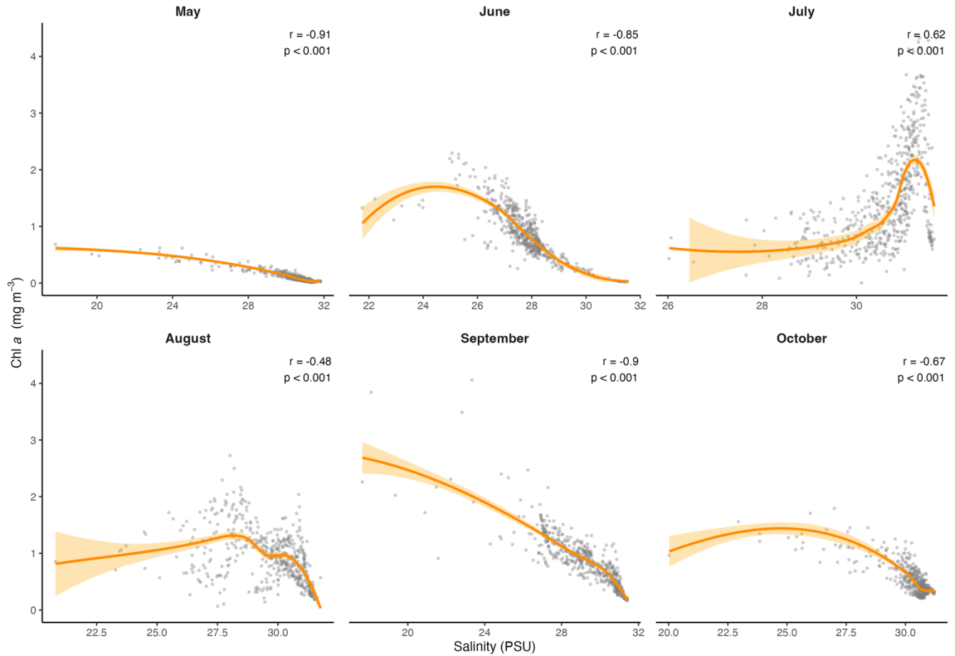
505 Figure A2: Scatter plots showing the monthly relationships between Chl a and salinity, across the transect. The orange line represents the LOESS curve with 95% confidence interval (shaded area). The Spearman correlation ( r ) and its p -value are also indicated.
