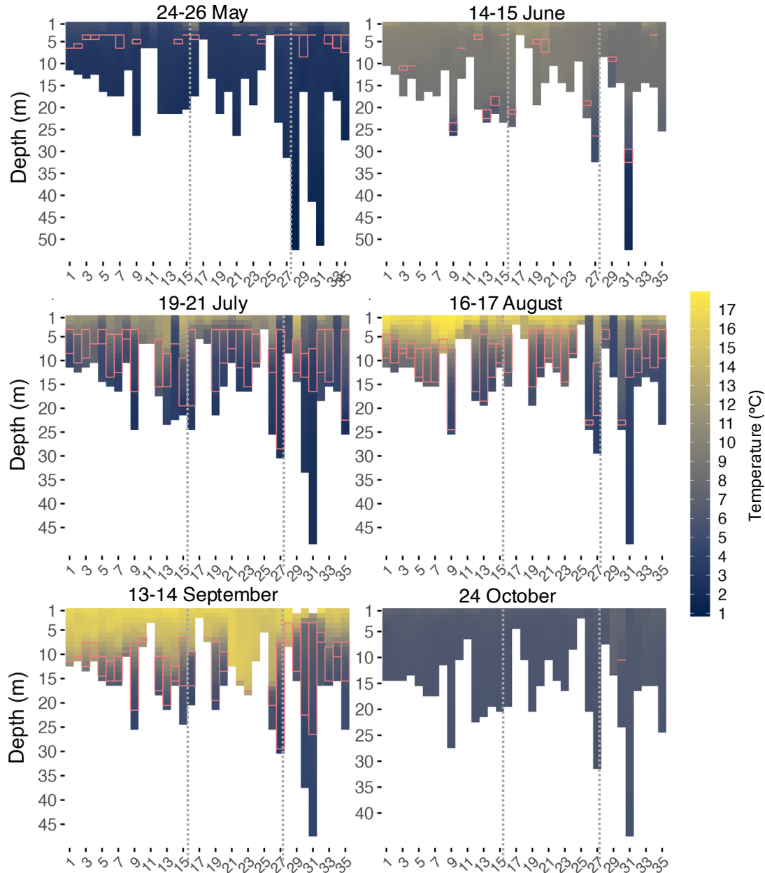
155 Figure 2: Temperature heatmaps for every month at every site (x axis) along the transect. Dotted lines indicate division of Zones 1 (West), 2 (BSI), and 3 (East), from left to right. The pink rectangles represent the thickness of the thermocline layer.
