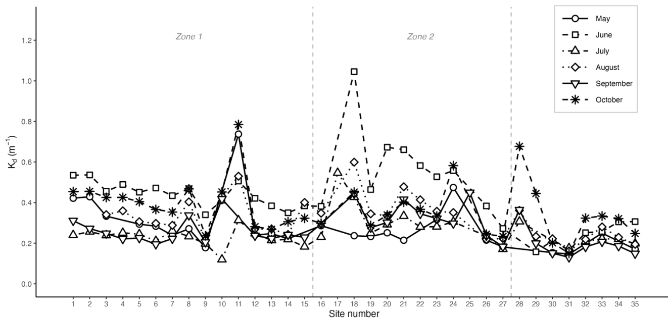
310 Figure 7: Diffuse light attenuation coefficient K_d at each site along the transect for the six sampling months. Dashed vertical lines 315 delimit the three site zones .
