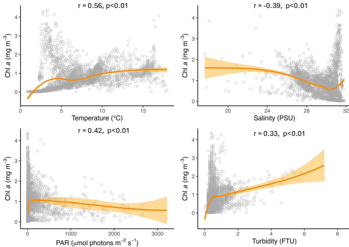
340 Figure 8: Scatter plots showing the relationships between Chl a and temperature, salinity, PAR and turbidity across the transect. The orange line represents the LOESS curve with 95% confidence interval (shaded area). The Spearman correlation ( r ) and its p-value are also indicated.
