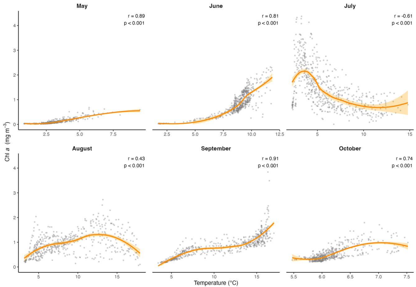
520 Figure A1: Scatter plots showing the monthly relationships between Chl a and temperature, across the transect. The orange line represents the LOESS curve with 95% confidence interval (shaded area). The Spearman correlation ( r ) and its p -value are also indicated.
