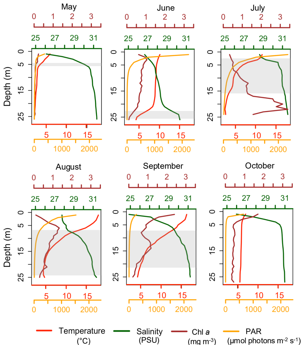
165 Figure 3: Vertical profiles of temperature, salinity, Chl a and PAR at Site 9, on each sampling date. The gray box represents the thermocline layer.
